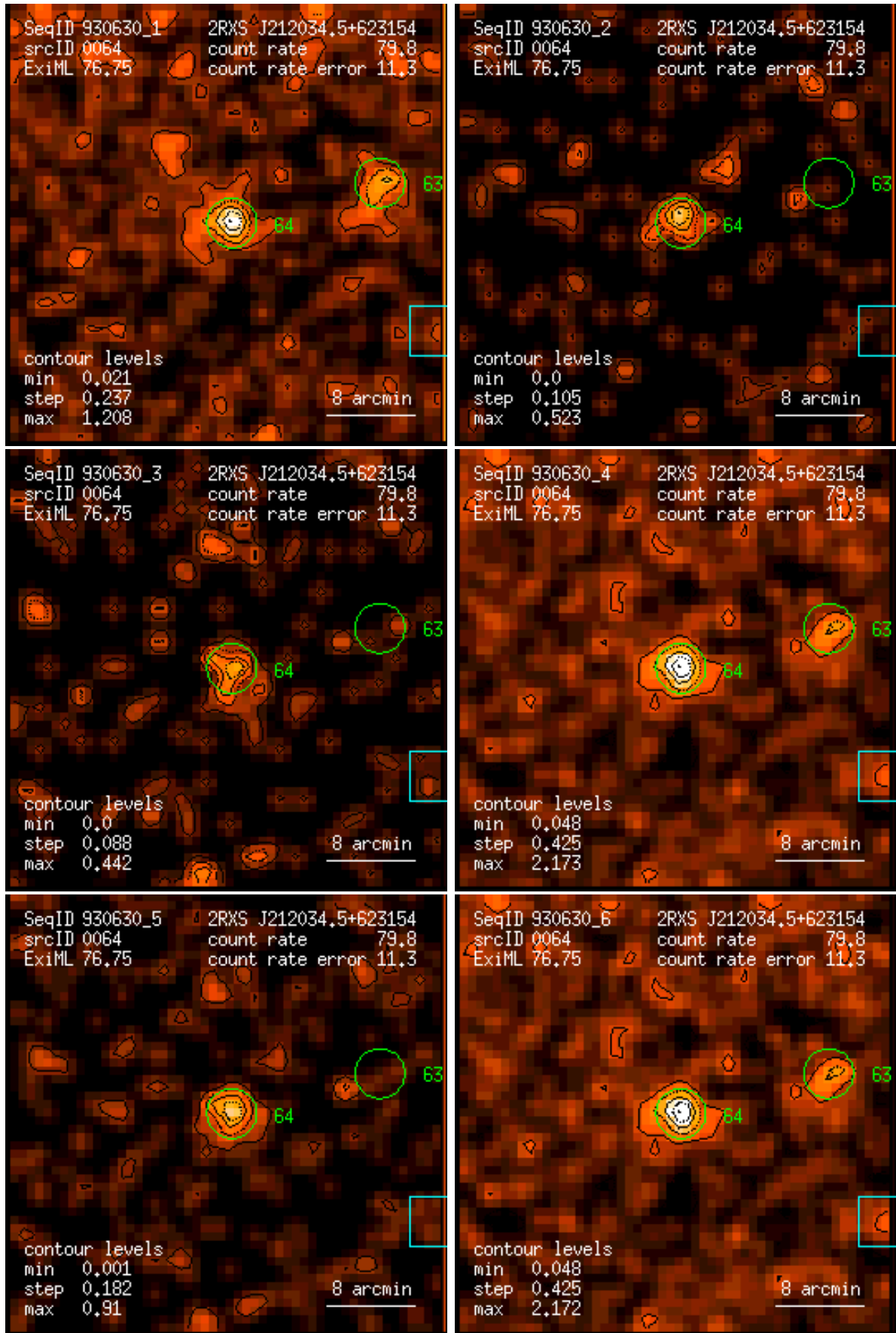
Figure 64: RASS 930630: detection 0064: band rate images, Gaussian filter: (1) PSPC channels 11 – 41, (2) 52 – 90, (3) 91 – 201, (4) 11 – 235, (5) 52 – 201, (6) 11 – 201. Broad band rates in counts/ks. Band rate contour levels in counts/ks/arcmin 2 .
