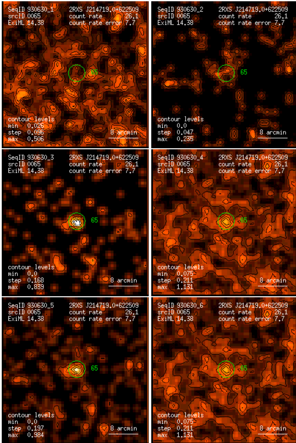
Figure 65: RASS 930630: detection 0065: band rate images, Gaussian filter: (1) PSPC channels 11 – 41, (2) 52 – 90, (3) 91 – 201, (4) 11 – 235, (5) 52 – 201, (6) 11 – 201. Broad band rates in counts/ks. Band rate contour levels in counts/ks/arcmin 2 .
