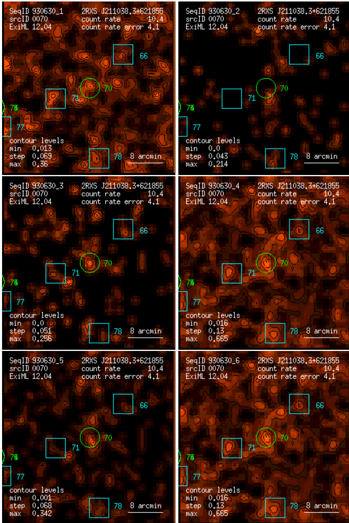
Figure 70: RASS 930630: detection 0070: band rate images, Gaussian filter: (1) PSPC channels 11 – 41, (2) 52 – 90, (3) 91 – 201, (4) 11 – 235, (5) 52 – 201, (6) 11 – 201. Broad band rates in counts/ks. Band rate contour levels in counts/ks/arcmin 2 .
