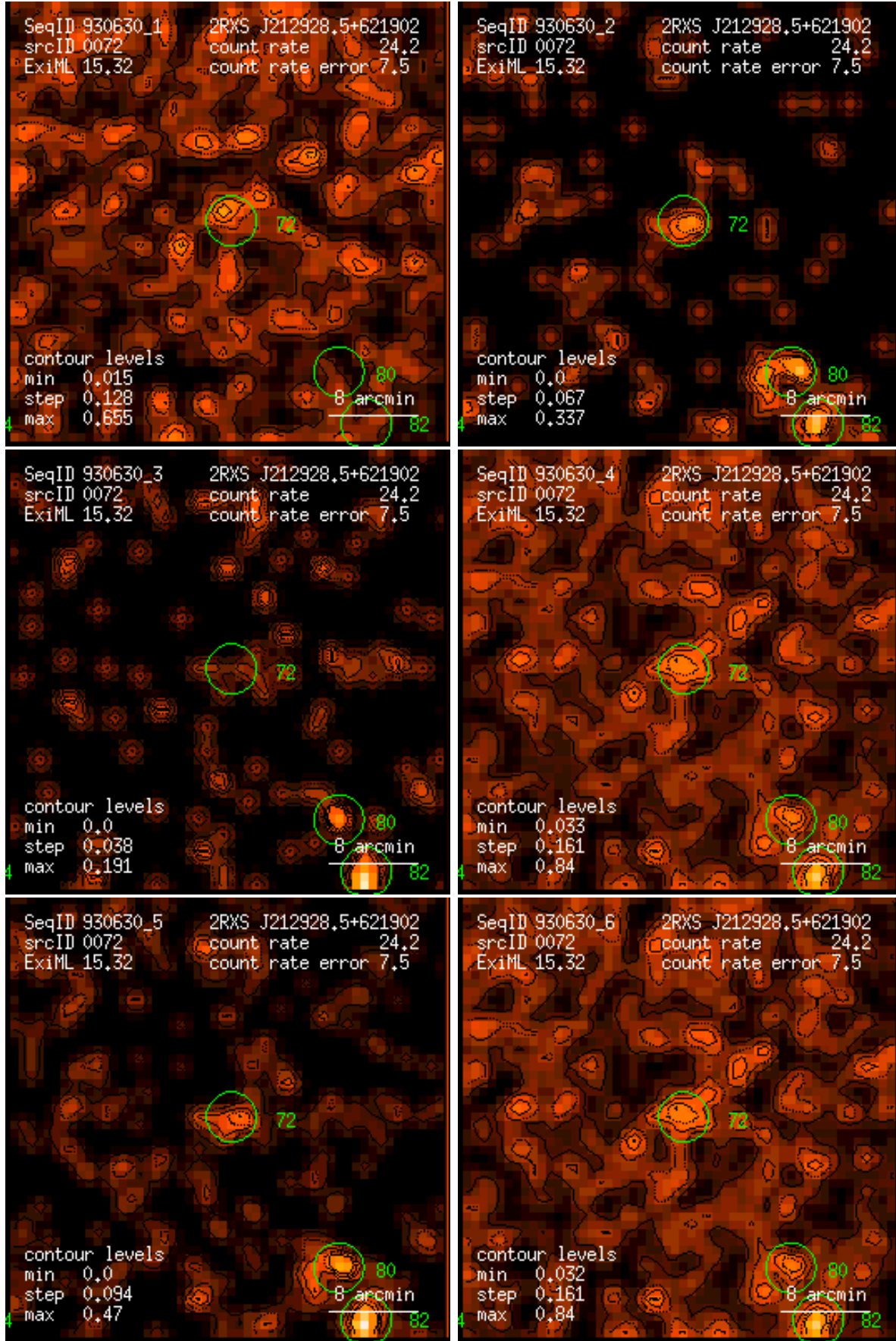
Figure 72: RASS 930630: detection 0072: band rate images, Gaussian filter: (1) PSPC channels 11 – 41, (2) 52 – 90, (3) 91 – 201, (4) 11 – 235, (5) 52 – 201, (6) 11 – 201. Broad band rates in counts/ks. Band rate contour levels in counts/ks/arcmin 2 .
