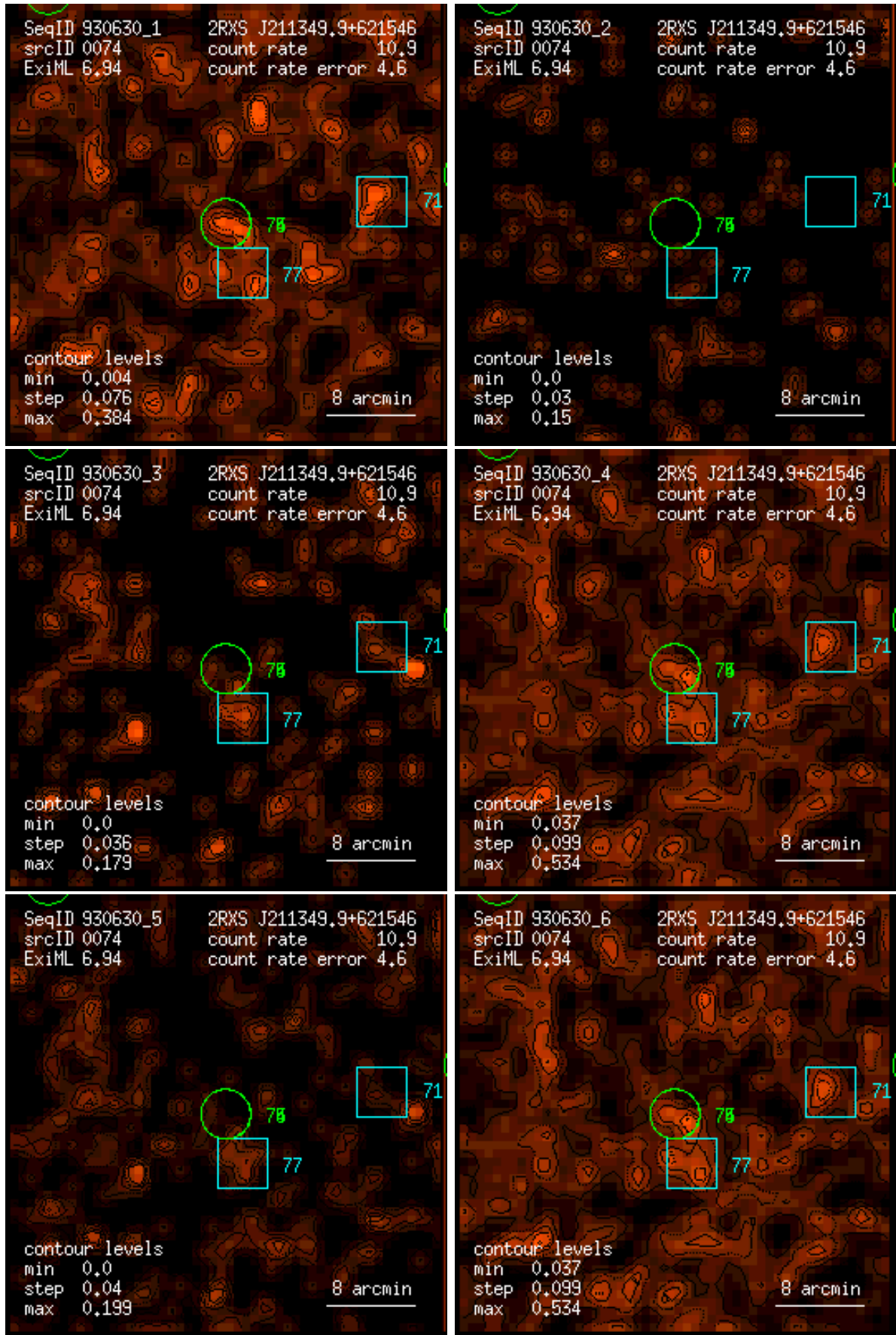
Figure 74: RASS 930630: detection 0074: band rate images, Gaussian filter: (1) PSPC channels 11 – 41, (2) 52 – 90, (3) 91 – 201, (4) 11 – 235, (5) 52 – 201, (6) 11 – 201. Broad band rates in counts/ks. Band rate contour levels in counts/ks/arcmin 2 .
