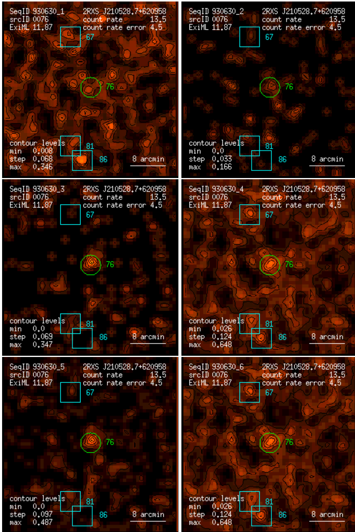
Figure 76: RASS 930630: detection 0076: band rate images, Gaussian filter: (1) PSPC channels 11 – 41, (2) 52 – 90, (3) 91 – 201, (4) 11 – 235, (5) 52 – 201, (6) 11 – 201. Broad band rates in counts/ks. Band rate contour levels in counts/ks/arcmin 2 .
