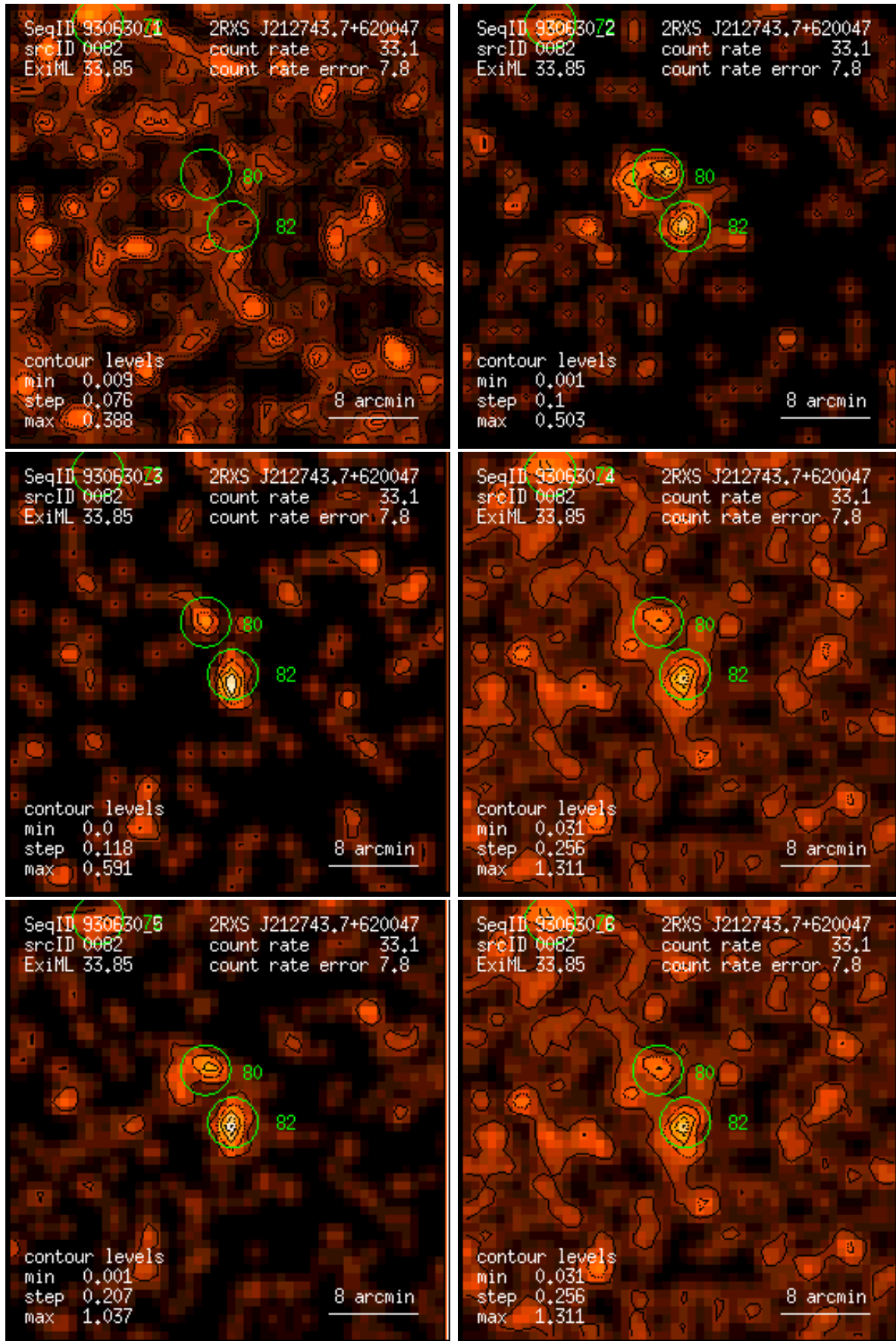
Figure 82: RASS 930630: detection 0082: band rate images, Gaussian filter: (1) PSPC channels 11 – 41, (2) 52 – 90, (3) 91 – 201, (4) 11 – 235, (5) 52 – 201, (6) 11 – 201. Broad band rates in counts/ks. Band rate contour levels in counts/ks/arcmin 2 .
