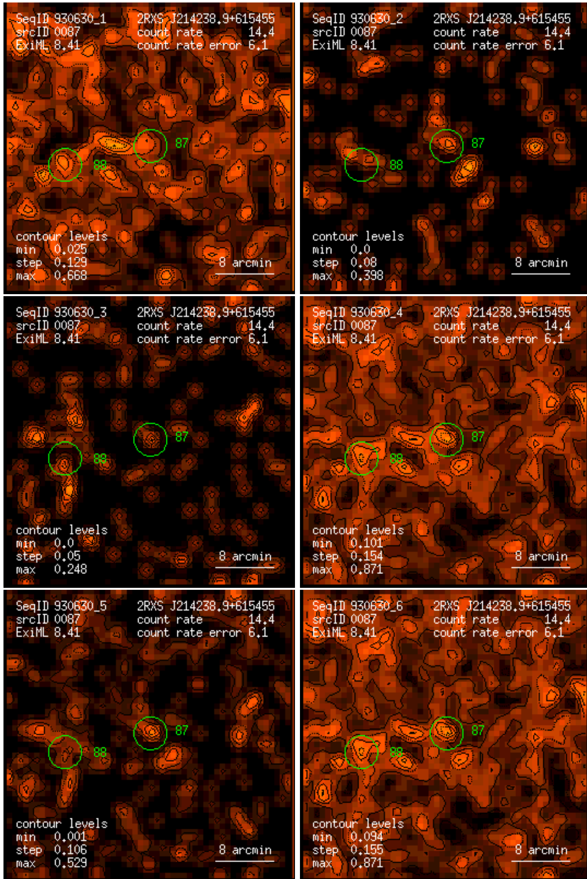
Figure 87: RASS 930630: detection 0087: band rate images, Gaussian filter: (1) PSPC channels 11 – 41, (2) 52 – 90, (3) 91 – 201, (4) 11 – 235, (5) 52 – 201, (6) 11 – 201. Broad band rates in counts/ks. Band rate contour levels in counts/ks/arcmin 2 .
