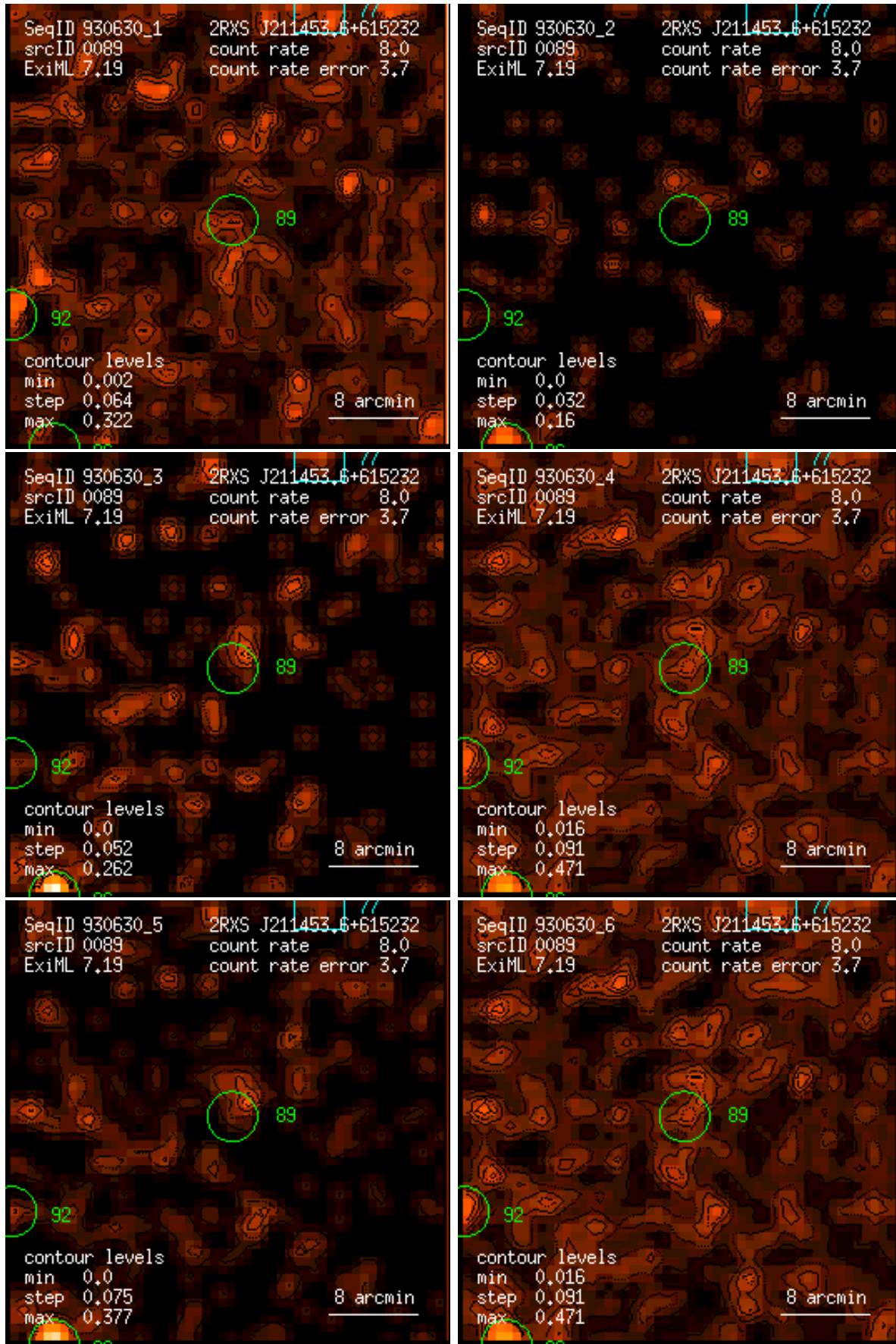
Figure 89: RASS 930630: detection 0089: band rate images, Gaussian filter: (1) PSPC channels 11 – 41, (2) 52 – 90, (3) 91 – 201, (4) 11 – 235, (5) 52 – 201, (6) 11 – 201. Broad band rates in counts/ks. Band rate contour levels in counts/ks/arcmin 2 .
