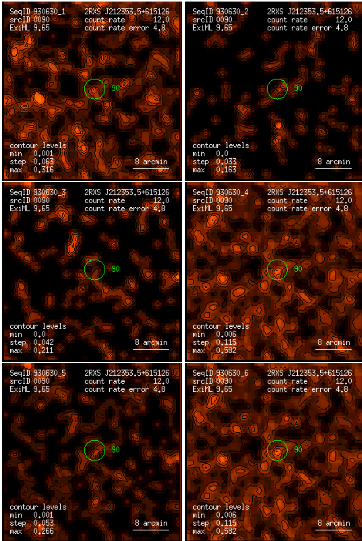
Figure 90: RASS 930630: detection 0090: band rate images, Gaussian filter: (1) PSPC channels 11 – 41, (2) 52 – 90, (3) 91 – 201, (4) 11 – 235, (5) 52 – 201, (6) 11 – 201. Broad band rates in counts/ks. Band rate contour levels in counts/ks/arcmin 2 .
