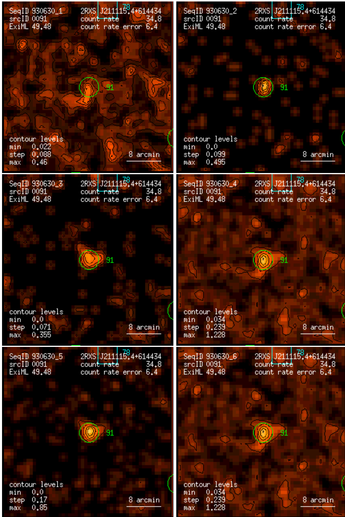
Figure 91: RASS 930630: detection 0091: band rate images, Gaussian filter: (1) PSPC channels 11 – 41, (2) 52 – 90, (3) 91 – 201, (4) 11 – 235, (5) 52 – 201, (6) 11 – 201. Broad band rates in counts/ks. Band rate contour levels in counts/ks/arcmin 2 .
