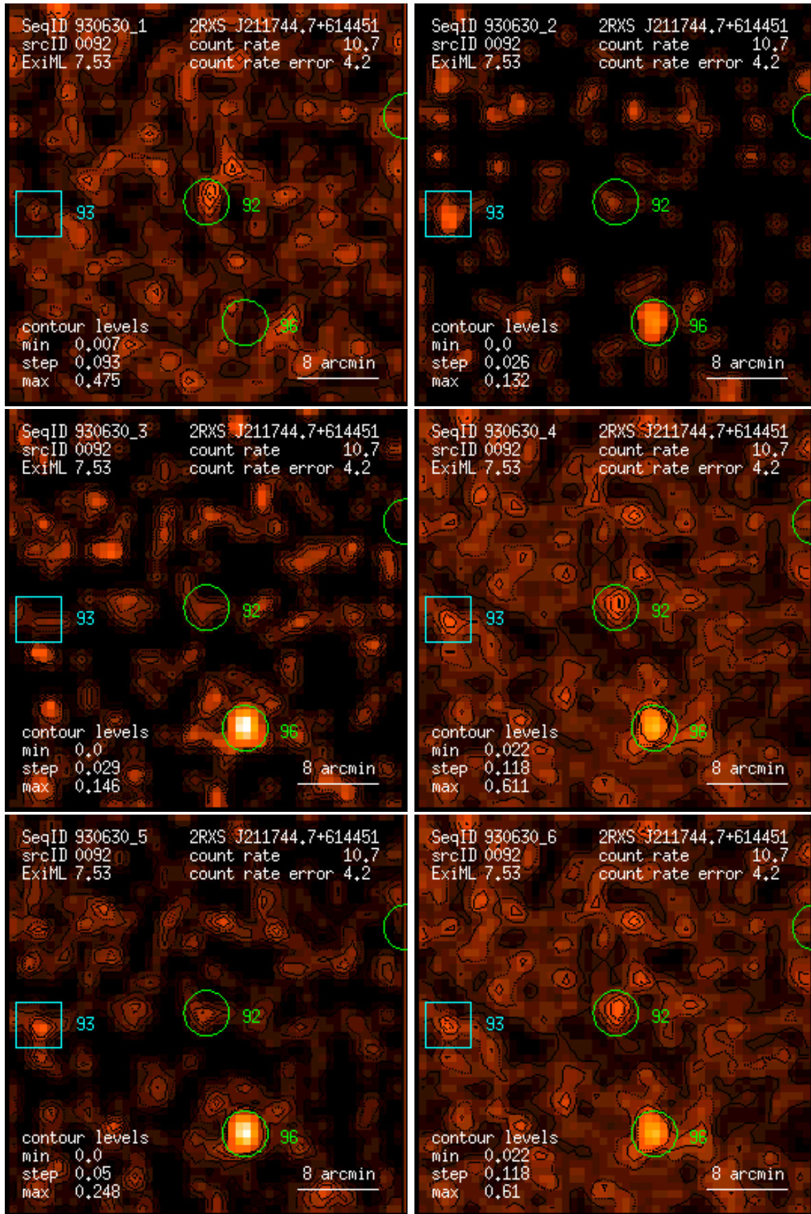
Figure 92: RASS 930630: detection 0092: band rate images, Gaussian filter: (1) PSPC channels 11 – 41, (2) 52 – 90, (3) 91 – 201, (4) 11 – 235, (5) 52 – 201, (6) 11 – 201. Broad band rates in counts/ks. Band rate contour levels in counts/ks/arcmin 2 .
