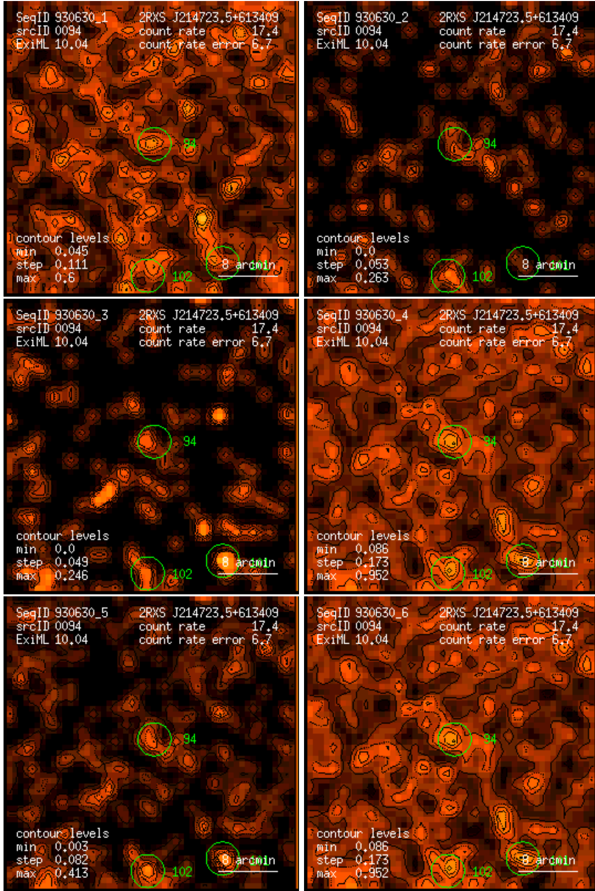
Figure 94: RASS 930630: detection 0094: band rate images, Gaussian filter: (1) PSPC channels 11 – 41, (2) 52 – 90, (3) 91 – 201, (4) 11 – 235, (5) 52 – 201, (6) 11 – 201. Broad band rates in counts/ks. Band rate contour levels in counts/ks/arcmin 2 .
