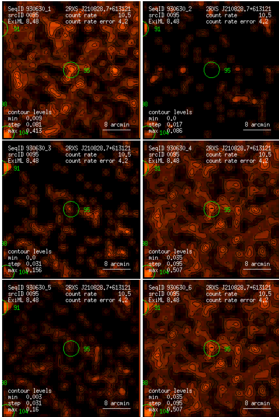
Figure 95: RASS 930630: detection 0095: band rate images, Gaussian filter: (1) PSPC channels 11 – 41, (2) 52 – 90, (3) 91 – 201, (4) 11 – 235, (5) 52 – 201, (6) 11 – 201. Broad band rates in counts/ks. Band rate contour levels in counts/ks/arcmin 2 .
