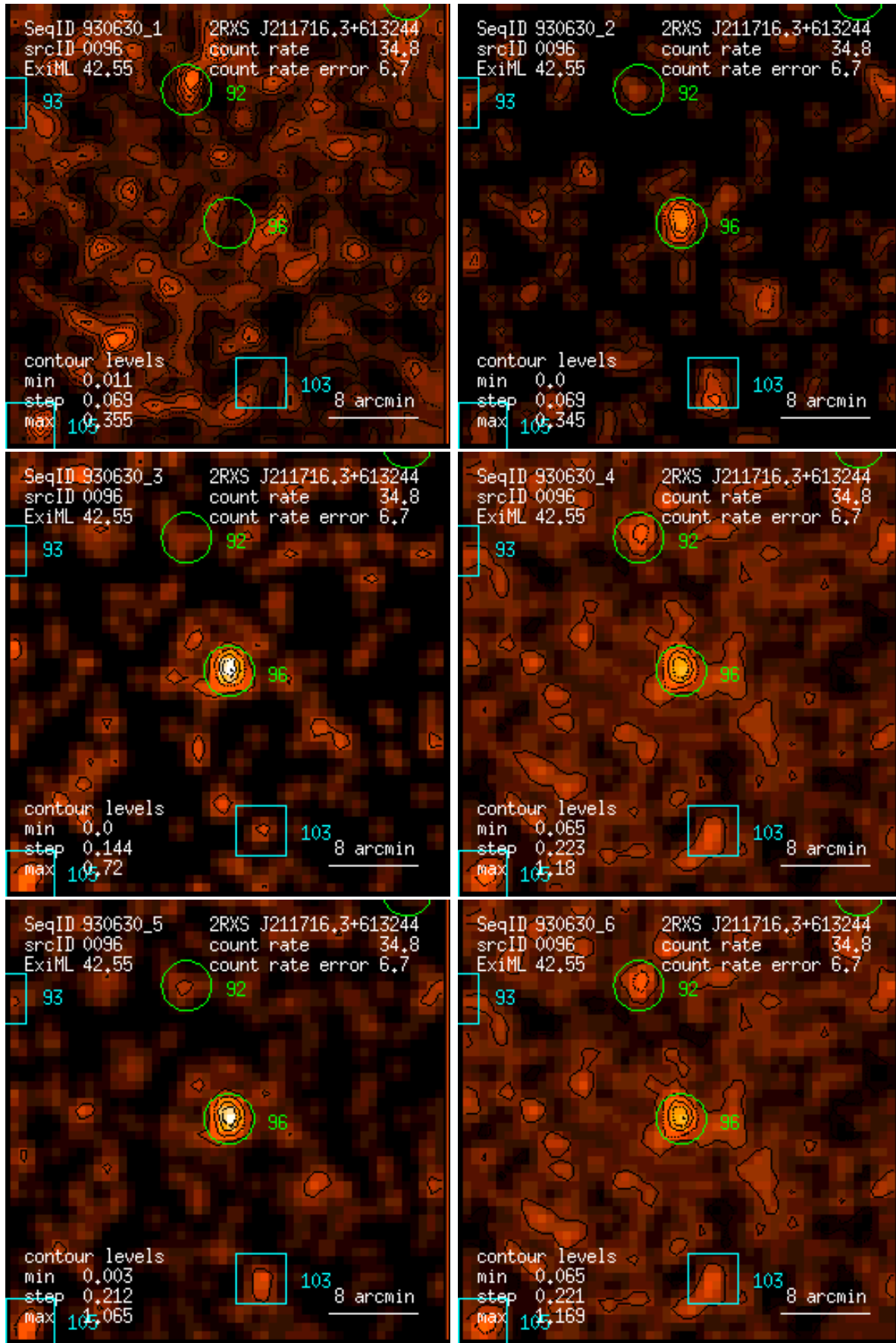
Figure 96: RASS 930630: detection 0096: band rate images, Gaussian filter: (1) PSPC channels 11 – 41, (2) 52 – 90, (3) 91 – 201, (4) 11 – 235, (5) 52 – 201, (6) 11 – 201. Broad band rates in counts/ks. Band rate contour levels in counts/ks/arcmin 2 .
