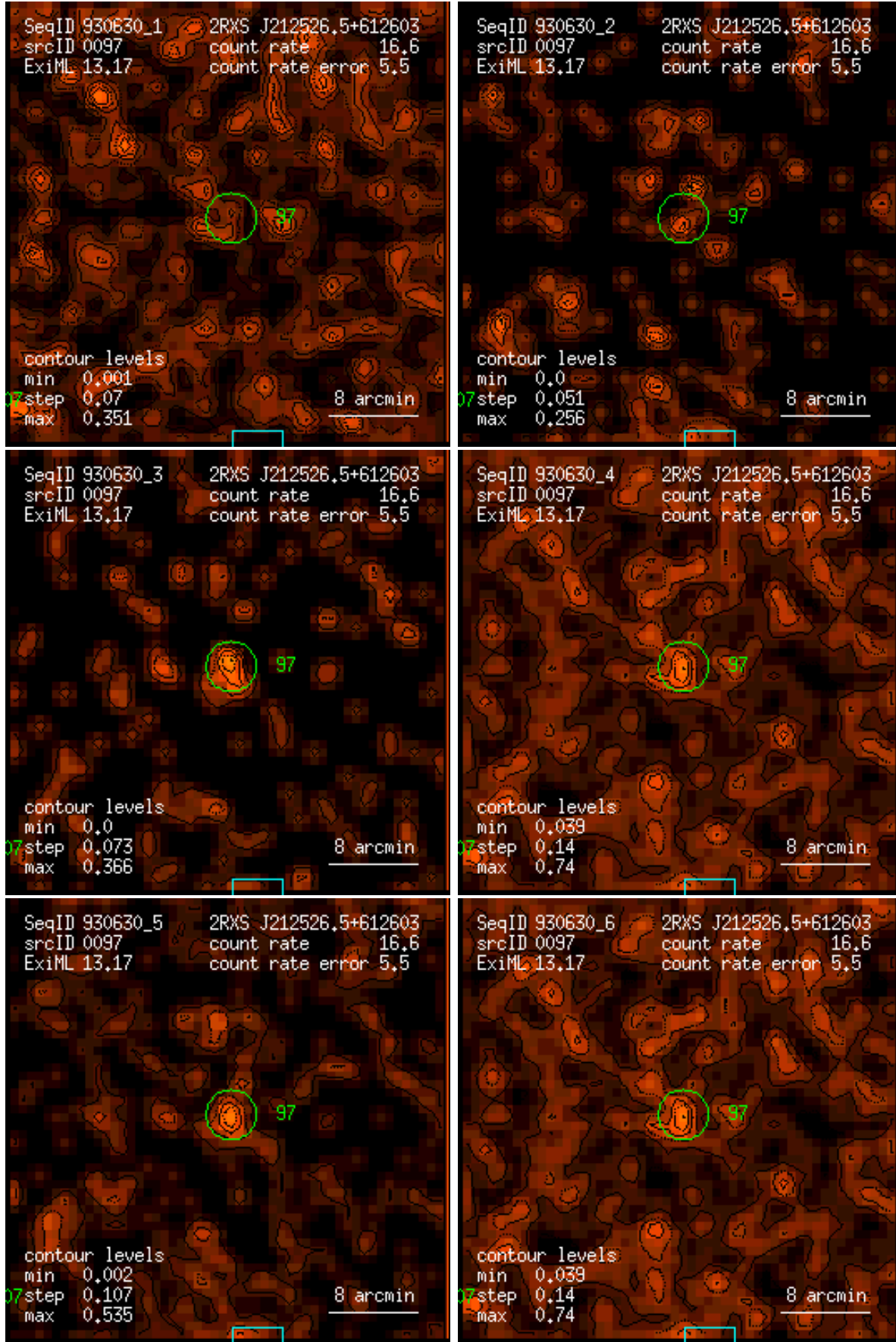
Figure 97: RASS 930630: detection 0097: band rate images, Gaussian filter: (1) PSPC channels 11 – 41, (2) 52 – 90, (3) 91 – 201, (4) 11 – 235, (5) 52 – 201, (6) 11 – 201. Broad band rates in counts/ks. Band rate contour levels in counts/ks/arcmin 2 .
