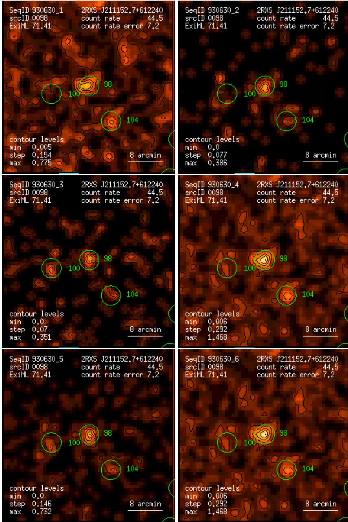
Figure 98: RASS 930630: detection 0098: band rate images, Gaussian filter: (1) PSPC channels 11 – 41, (2) 52 – 90, (3) 91 – 201, (4) 11 – 235, (5) 52 – 201, (6) 11 – 201. Broad band rates in counts/ks. Band rate contour levels in counts/ks/arcmin 2 .
