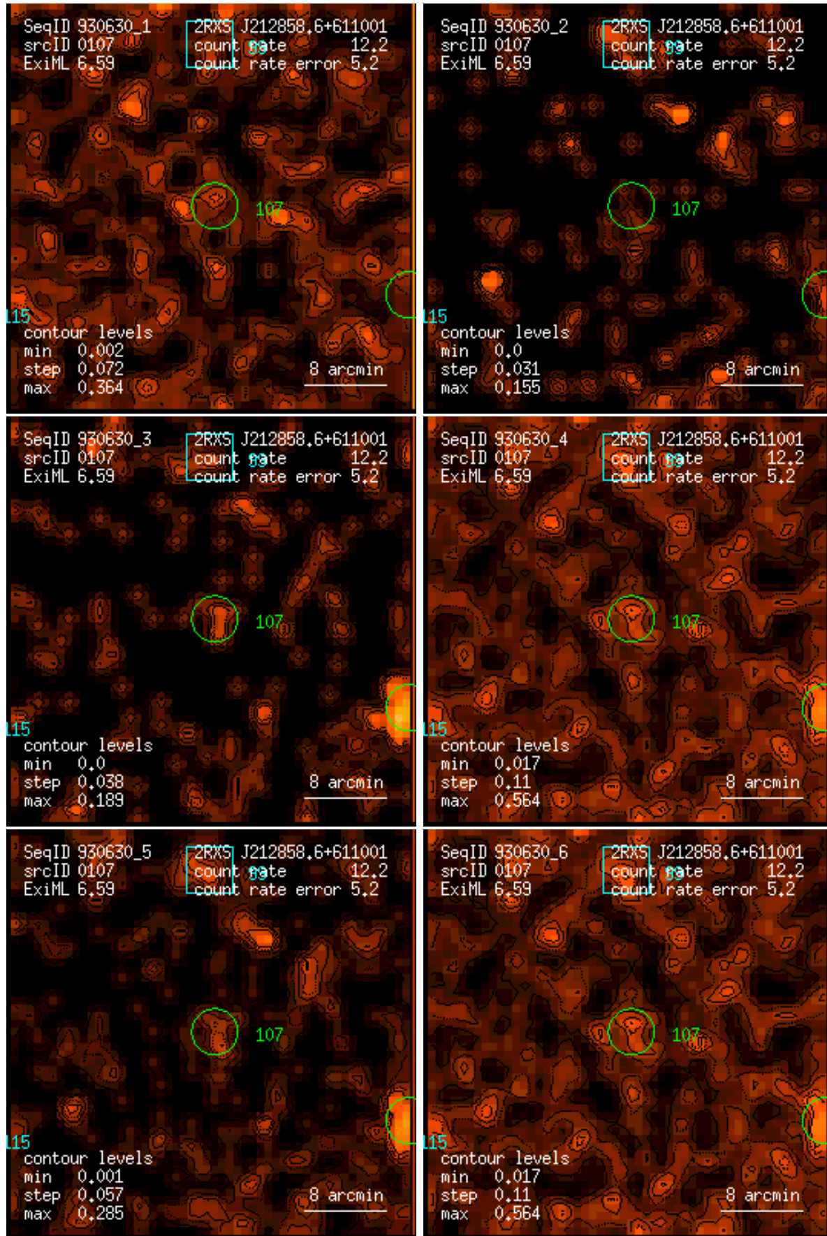
Figure 107: RASS 930630: detection 0107: band rate images, Gaussian filter: (1) PSPC channels 11 – 41, (2) 52 – 90, (3) 91 – 201, (4) 11 – 235, (5) 52 – 201, (6) 11 – 201. Broad band rates in counts/ks. Band rate contour levels in counts/ks/arcmin 2 .
