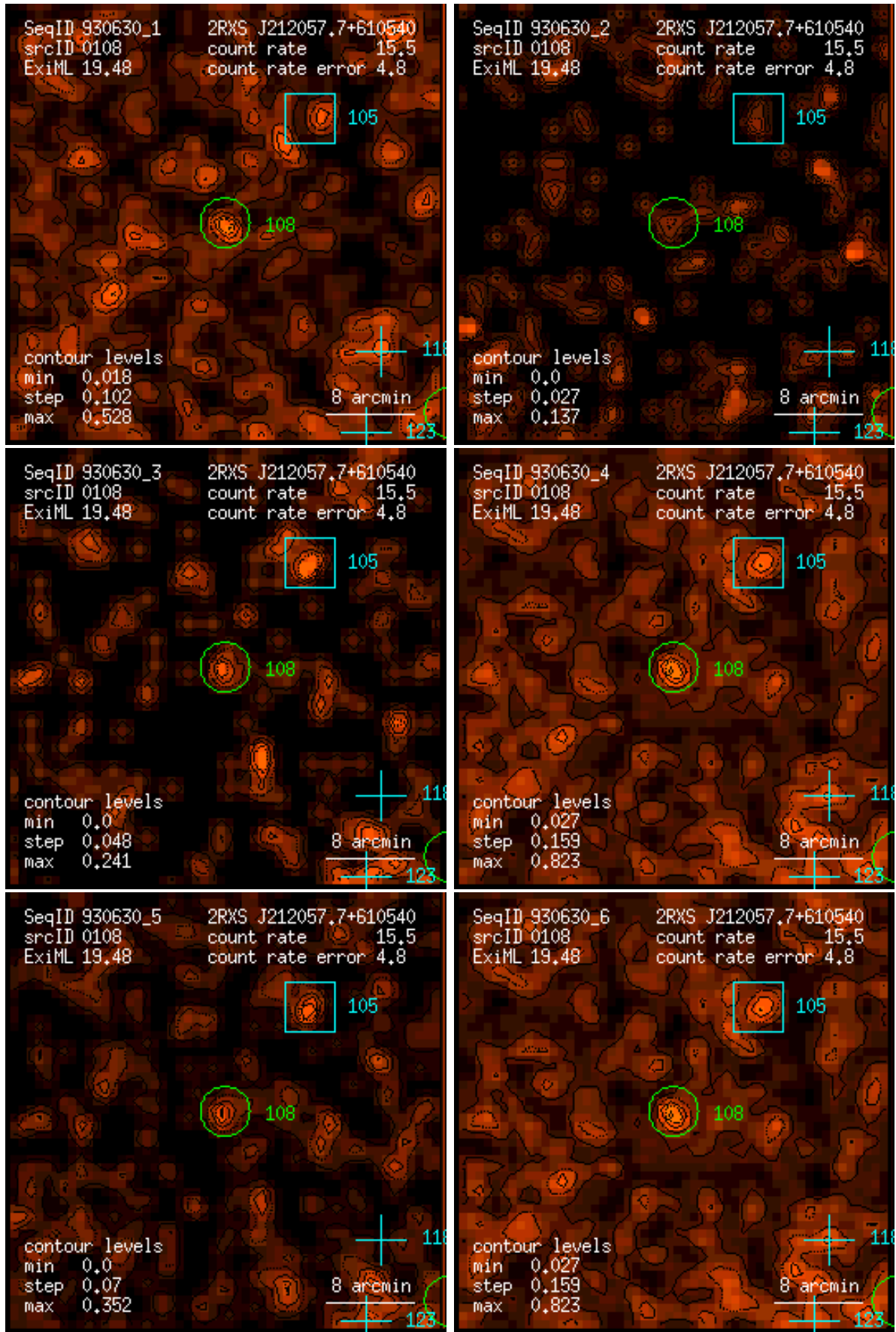
Figure 108: RASS 930630: detection 0108: band rate images, Gaussian filter: (1) PSPC channels 11 – 41, (2) 52 – 90, (3) 91 – 201, (4) 11 – 235, (5) 52 – 201, (6) 11 – 201. Broad band rates in counts/ks. Band rate contour levels in counts/ks/arcmin 2 .
