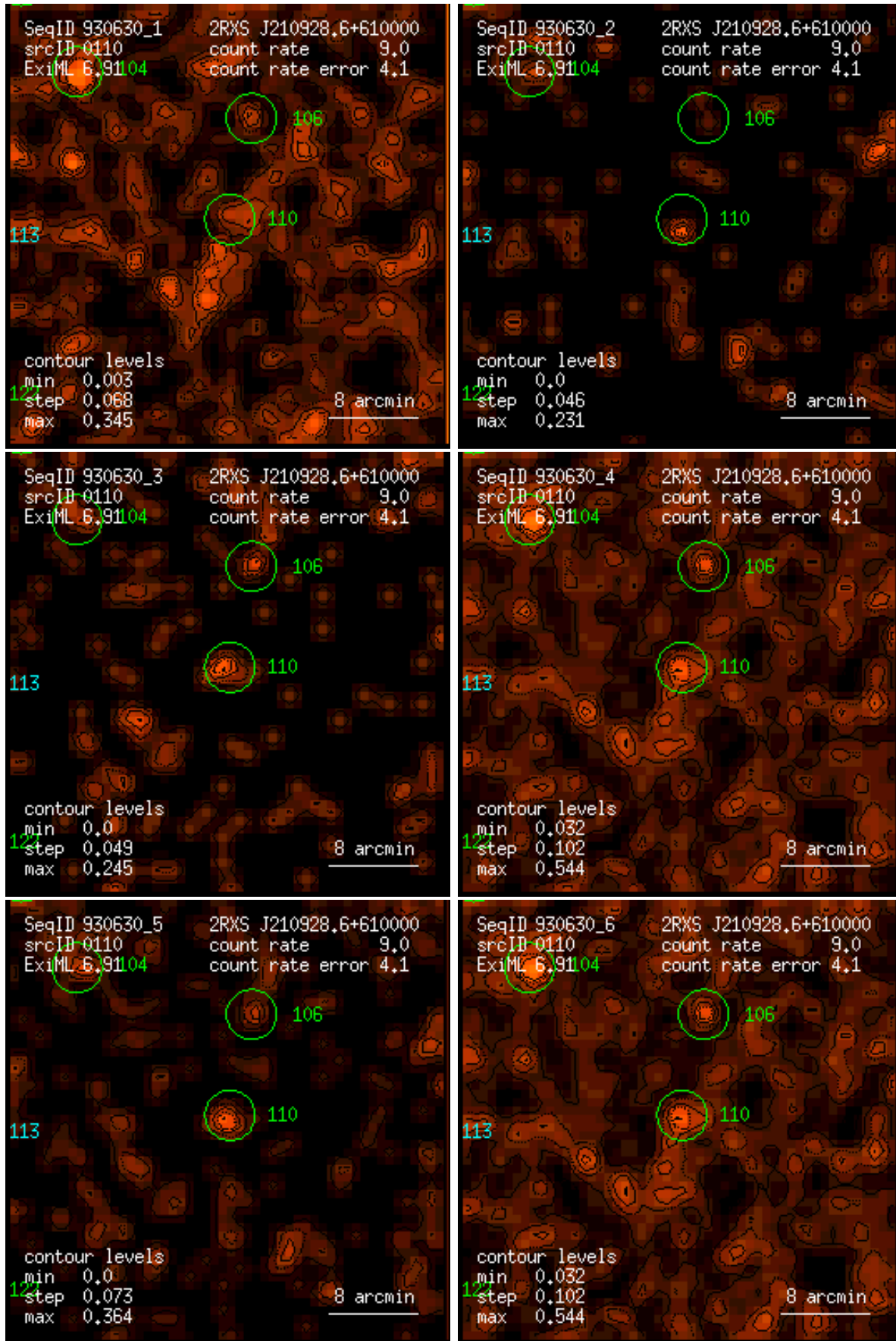
Figure 110: RASS 930630: detection 0110: band rate images, Gaussian filter: (1) PSPC channels 11 – 41, (2) 52 – 90, (3) 91 – 201, (4) 11 – 235, (5) 52 – 201, (6) 11 – 201. Broad band rates in counts/ks. Band rate contour levels in counts/ks/arcmin 2 .
