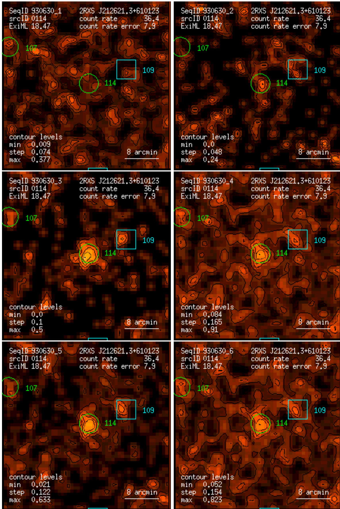
Figure 114: RASS 930630: detection 0114: band rate images, Gaussian filter: (1) PSPC channels 11 – 41, (2) 52 – 90, (3) 91 – 201, (4) 11 – 235, (5) 52 – 201, (6) 11 – 201. Broad band rates in counts/ks. Band rate contour levels in counts/ks/arcmin 2 .
