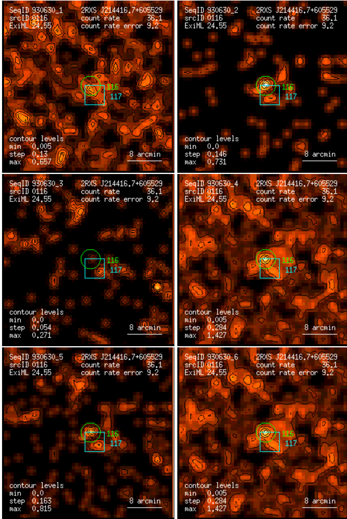
Figure 116: RASS 930630: detection 0116: band rate images, Gaussian filter: (1) PSPC channels 11 – 41, (2) 52 – 90, (3) 91 – 201, (4) 11 – 235, (5) 52 – 201, (6) 11 – 201. Broad band rates in counts/ks. Band rate contour levels in counts/ks/arcmin 2 .
