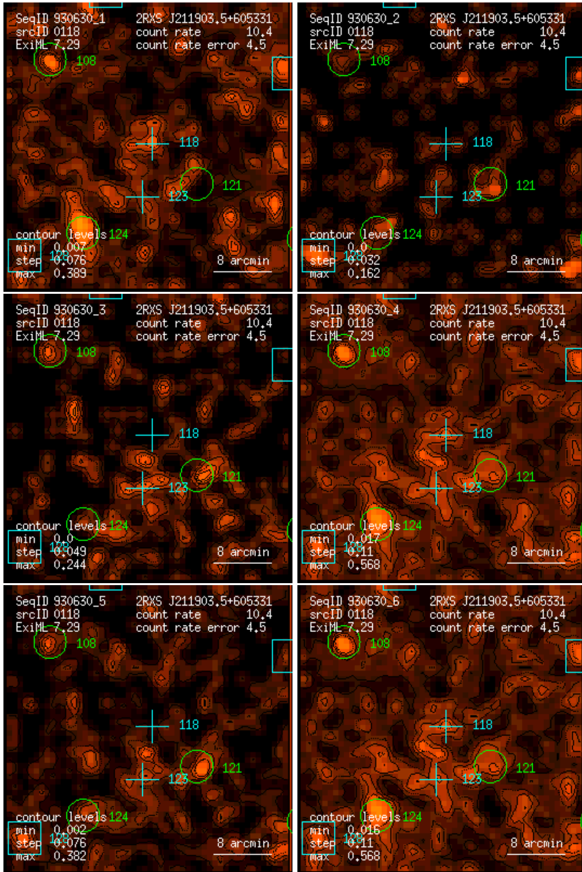
Figure 118: RASS 930630: detection 0118: band rate images, Gaussian filter: (1) PSPC channels 11 – 41, (2) 52 – 90, (3) 91 – 201, (4) 11 – 235, (5) 52 – 201, (6) 11 – 201. Broad band rates in counts/ks. Band rate contour levels in counts/ks/arcmin 2 .
