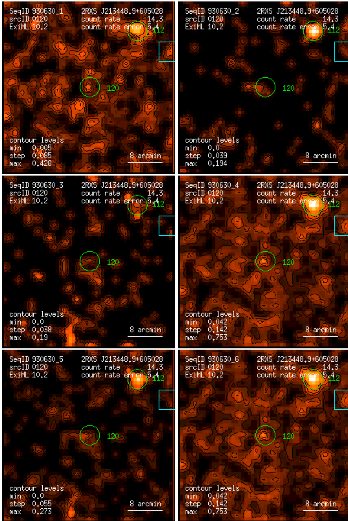
Figure 120: RASS 930630: detection 0120: band rate images, Gaussian filter: (1) PSPC channels 11 – 41, (2) 52 – 90, (3) 91 – 201, (4) 11 – 235, (5) 52 – 201, (6) 11 – 201. Broad band rates in counts/ks. Band rate contour levels in counts/ks/arcmin 2 .
