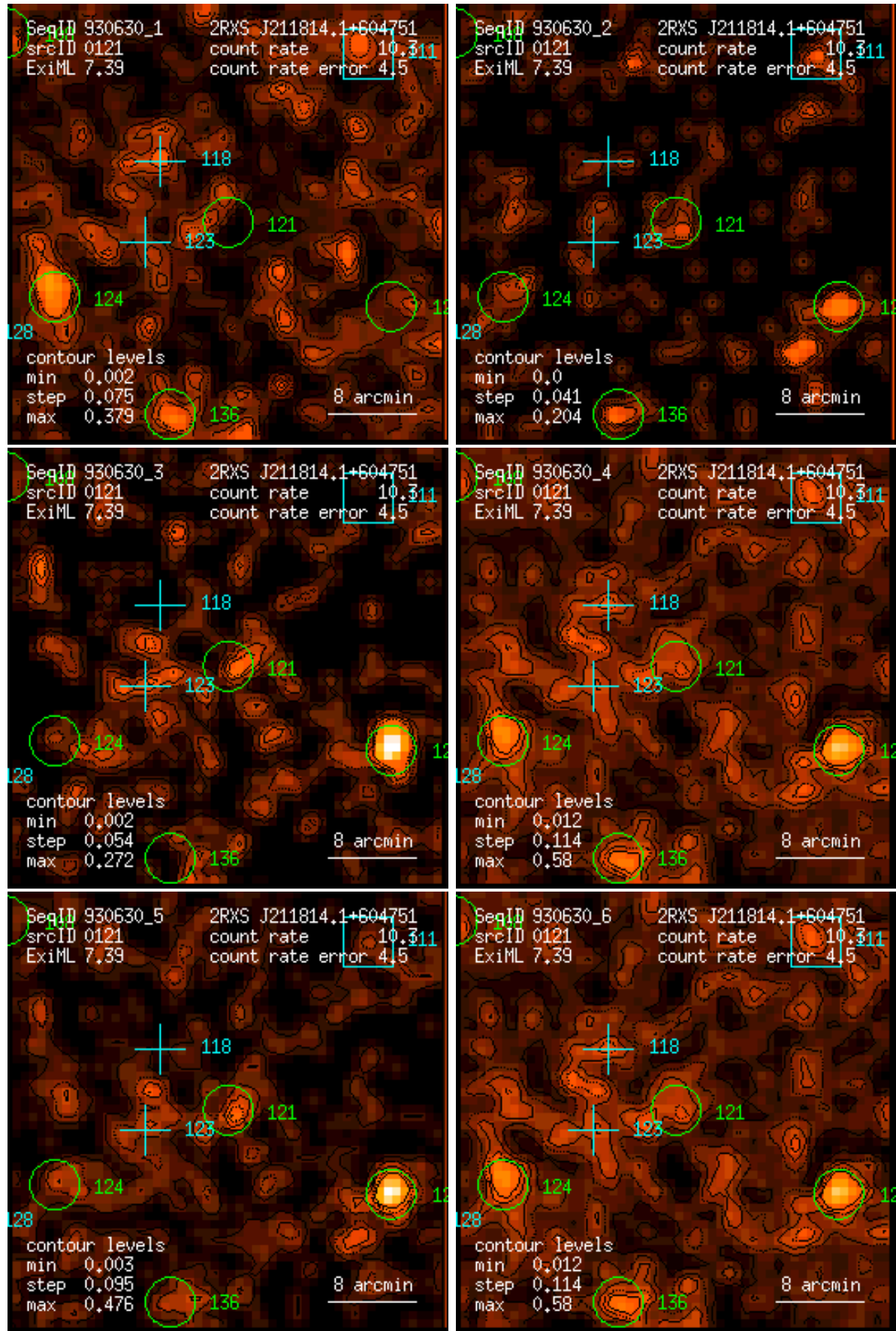
Figure 121: RASS 930630: detection 0121: band rate images, Gaussian filter: (1) PSPC channels 11 – 41, (2) 52 – 90, (3) 91 – 201, (4) 11 – 235, (5) 52 – 201, (6) 11 – 201. Broad band rates in counts/ks. Band rate contour levels in counts/ks/arcmin 2 .
