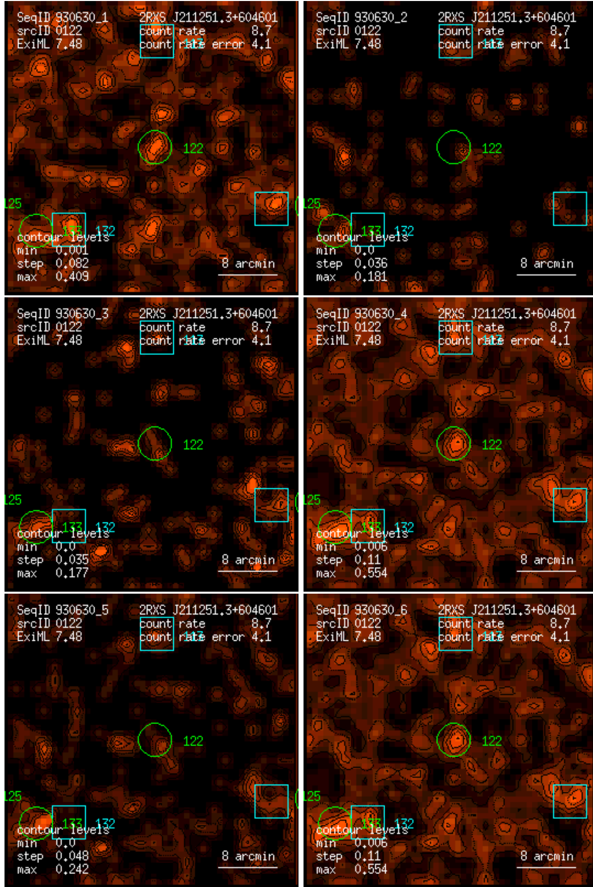
Figure 122: RASS 930630: detection 0122: band rate images, Gaussian filter: (1) PSPC channels 11 – 41, (2) 52 – 90, (3) 91 – 201, (4) 11 – 235, (5) 52 – 201, (6) 11 – 201. Broad band rates in counts/ks. Band rate contour levels in counts/ks/arcmin 2 .
