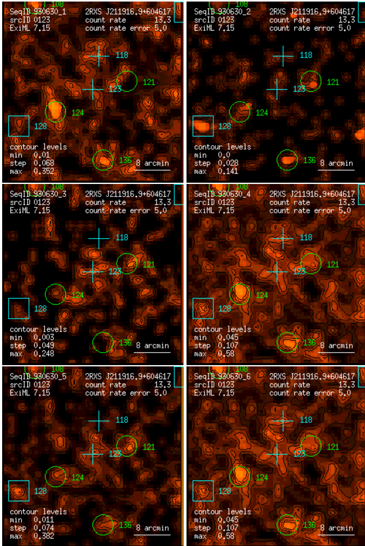
Figure 123: RASS 930630: detection 0123: band rate images, Gaussian filter: (1) PSPC channels 11 – 41, (2) 52 – 90, (3) 91 – 201, (4) 11 – 235, (5) 52 – 201, (6) 11 – 201. Broad band rates in counts/ks. Band rate contour levels in counts/ks/arcmin 2 .
