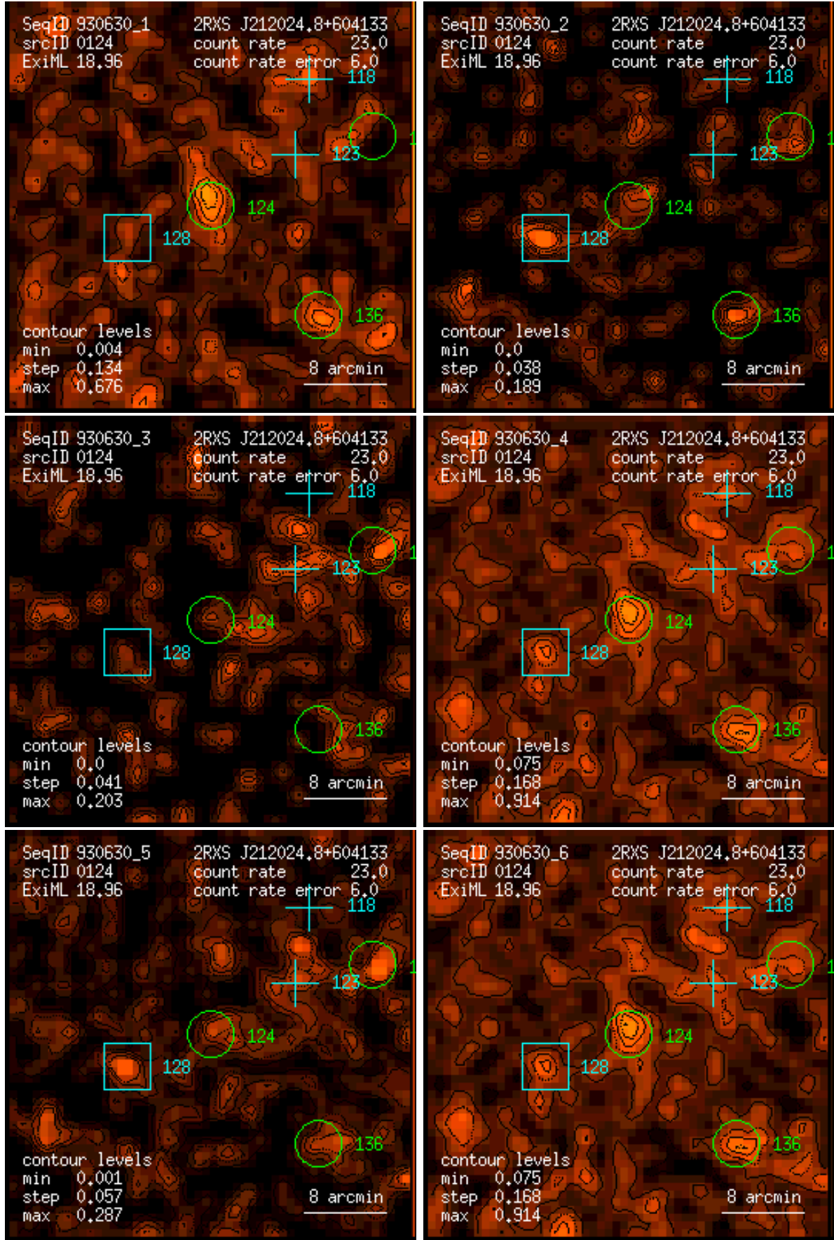
Figure 124: RASS 930630: detection 0124: band rate images, Gaussian filter: (1) PSPC channels 11 – 41, (2) 52 – 90, (3) 91 – 201, (4) 11 – 235, (5) 52 – 201, (6) 11 – 201. Broad band rates in counts/ks. Band rate contour levels in counts/ks/arcmin 2 .
