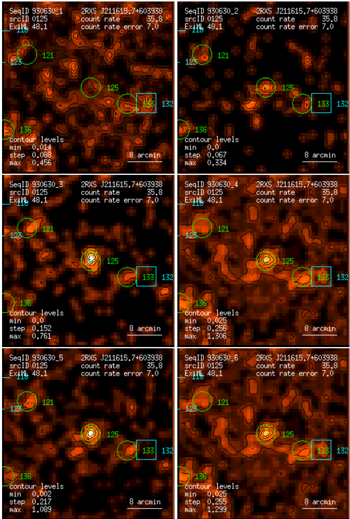
Figure 125: RASS 930630: detection 0125: band rate images, Gaussian filter: (1) PSPC channels 11 – 41, (2) 52 – 90, (3) 91 – 201, (4) 11 – 235, (5) 52 – 201, (6) 11 – 201. Broad band rates in counts/ks. Band rate contour levels in counts/ks/arcmin 2 .
