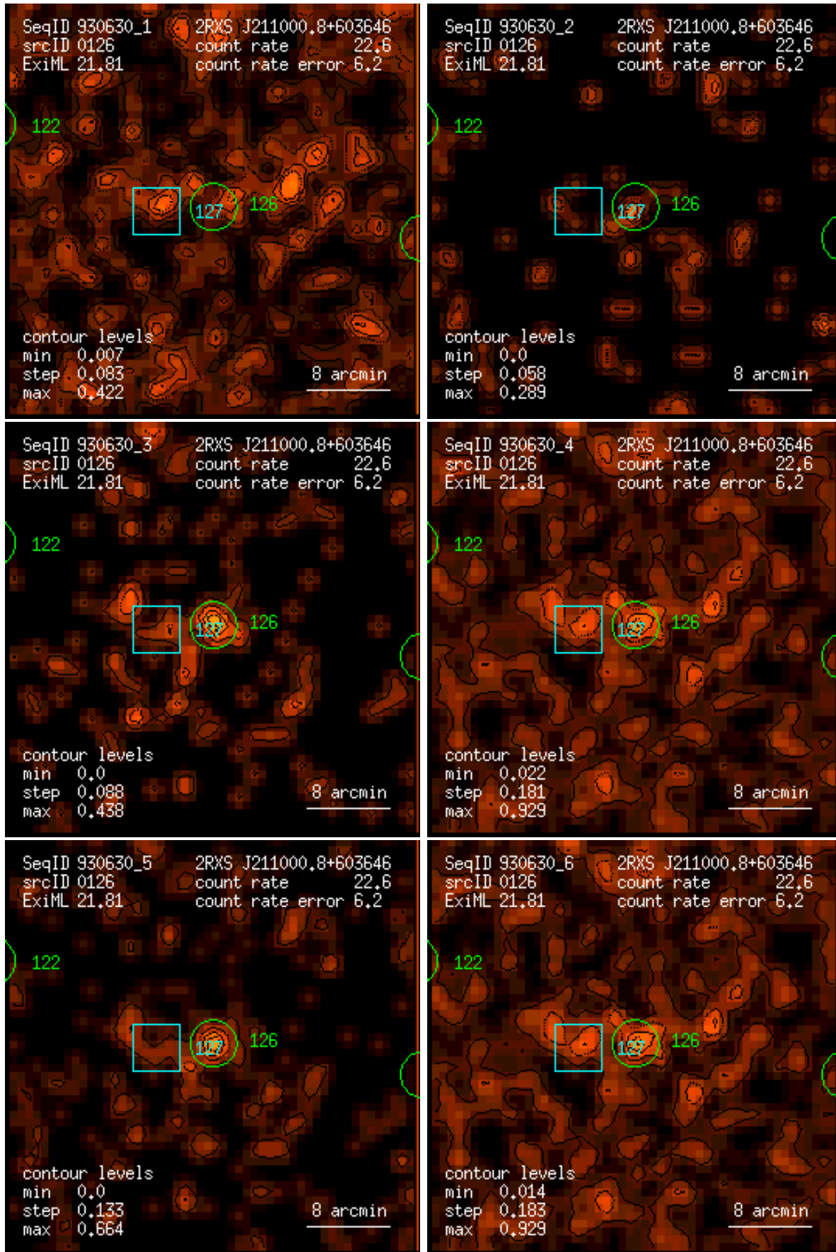
Figure 126: RASS 930630: detection 0126: band rate images, Gaussian filter: (1) PSPC channels 11 – 41, (2) 52 – 90, (3) 91 – 201, (4) 11 – 235, (5) 52 – 201, (6) 11 – 201. Broad band rates in counts/ks. Band rate contour levels in counts/ks/arcmin 2 .
