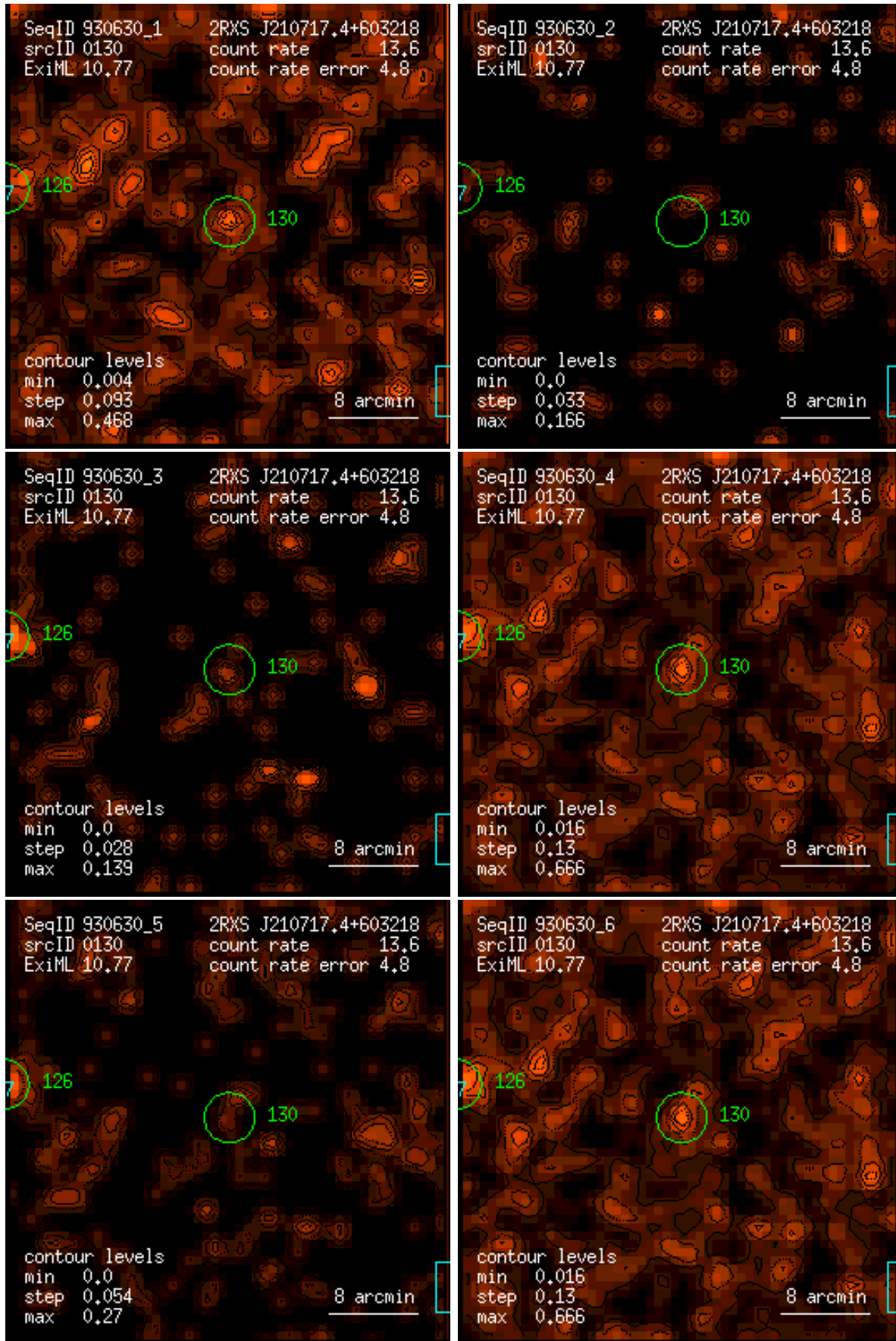
Figure 130: RASS 930630: detection 0130: band rate images, Gaussian filter: (1) PSPC channels 11 – 41, (2) 52 – 90, (3) 91 – 201, (4) 11 – 235, (5) 52 – 201, (6) 11 – 201. Broad band rates in counts/ks. Band rate contour levels in counts/ks/arcmin 2 .
