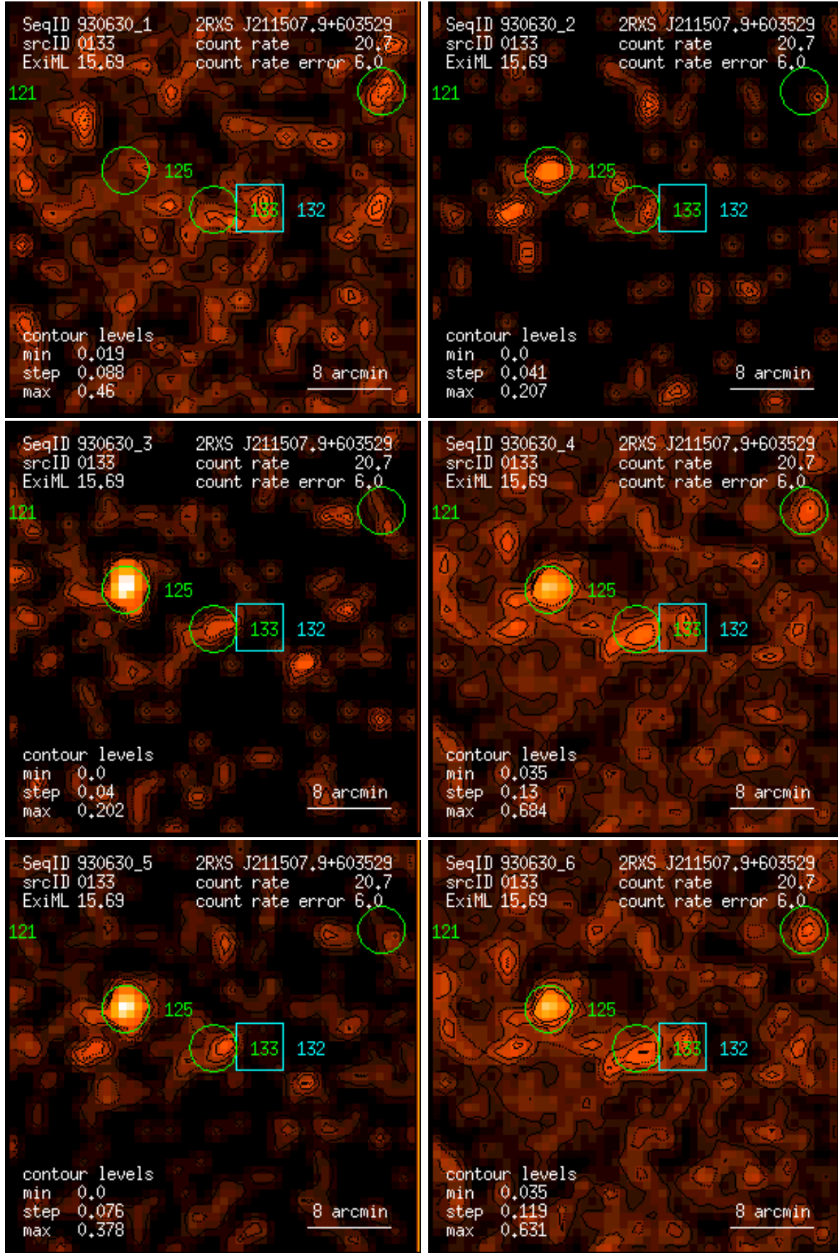
Figure 133: RASS 930630: detection 0133: band rate images, Gaussian filter: (1) PSPC channels 11 – 41, (2) 52 – 90, (3) 91 – 201, (4) 11 – 235, (5) 52 – 201, (6) 11 – 201. Broad band rates in counts/ks. Band rate contour levels in counts/ks/arcmin 2 .
