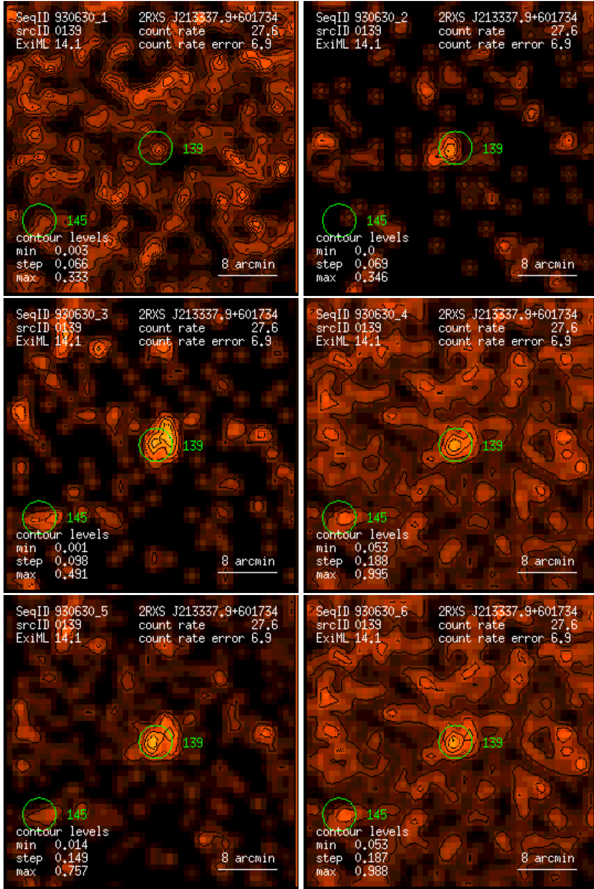
Figure 139: RASS 930630: detection 0139: band rate images, Gaussian filter: (1) PSPC channels 11 – 41, (2) 52 – 90, (3) 91 – 201, (4) 11 – 235, (5) 52 – 201, (6) 11 – 201. Broad band rates in counts/ks. Band rate contour levels in counts/ks/arcmin 2 .
