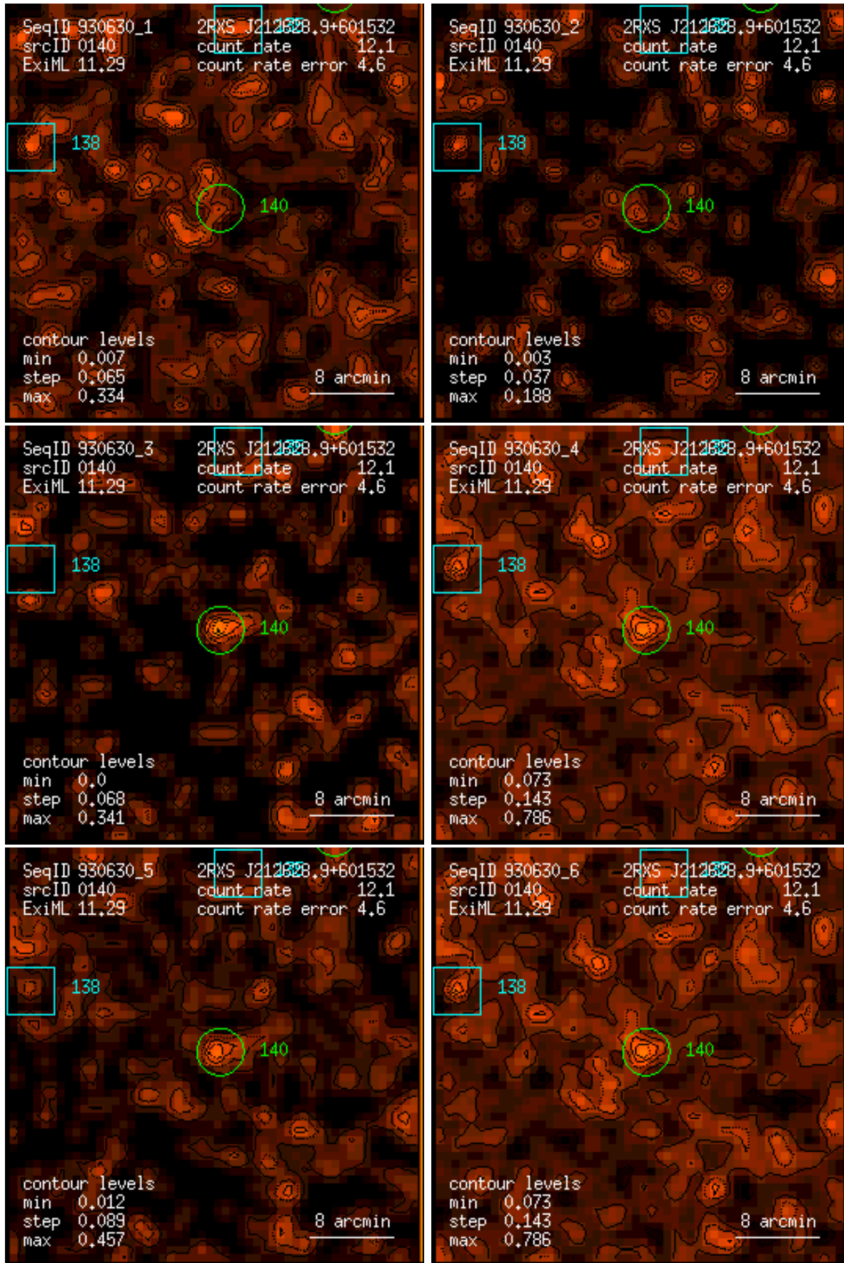
Figure 140: RASS 930630: detection 0140: band rate images, Gaussian filter: (1) PSPC channels 11 – 41, (2) 52 – 90, (3) 91 – 201, (4) 11 – 235, (5) 52 – 201, (6) 11 – 201. Broad band rates in counts/ks. Band rate contour levels in counts/ks/arcmin 2 .
