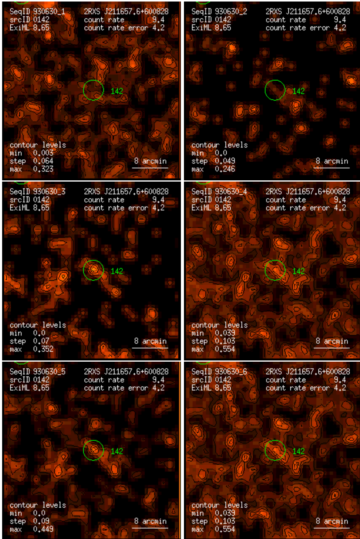
Figure 142: RASS 930630: detection 0142: band rate images, Gaussian filter: (1) PSPC channels 11 – 41, (2) 52 – 90, (3) 91 – 201, (4) 11 – 235, (5) 52 – 201, (6) 11 – 201. Broad band rates in counts/ks. Band rate contour levels in counts/ks/arcmin 2 .
