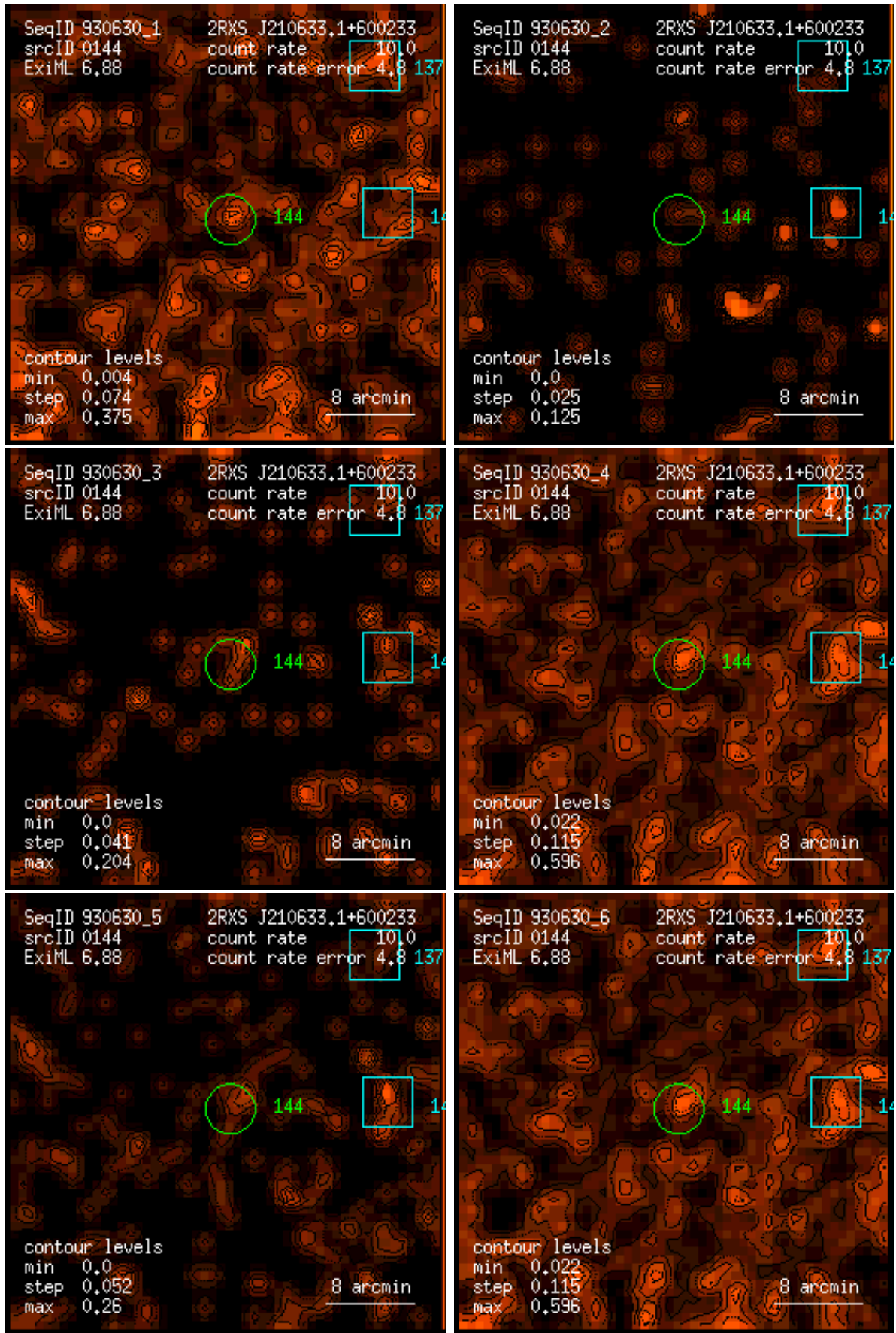
Figure 144: RASS 930630: detection 0144: band rate images, Gaussian filter: (1) PSPC channels 11 – 41, (2) 52 – 90, (3) 91 – 201, (4) 11 – 235, (5) 52 – 201, (6) 11 – 201. Broad band rates in counts/ks. Band rate contour levels in counts/ks/arcmin 2 .
