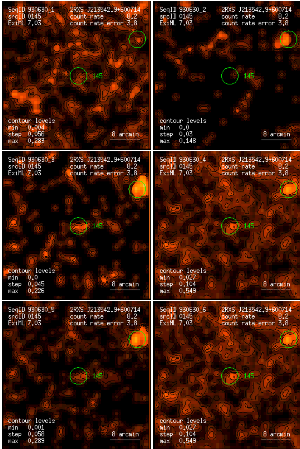
Figure 145: RASS 930630: detection 0145: band rate images, Gaussian filter: (1) PSPC channels 11 – 41, (2) 52 – 90, (3) 91 – 201, (4) 11 – 235, (5) 52 – 201, (6) 11 – 201. Broad band rates in counts/ks. Band rate contour levels in counts/ks/arcmin 2 .
