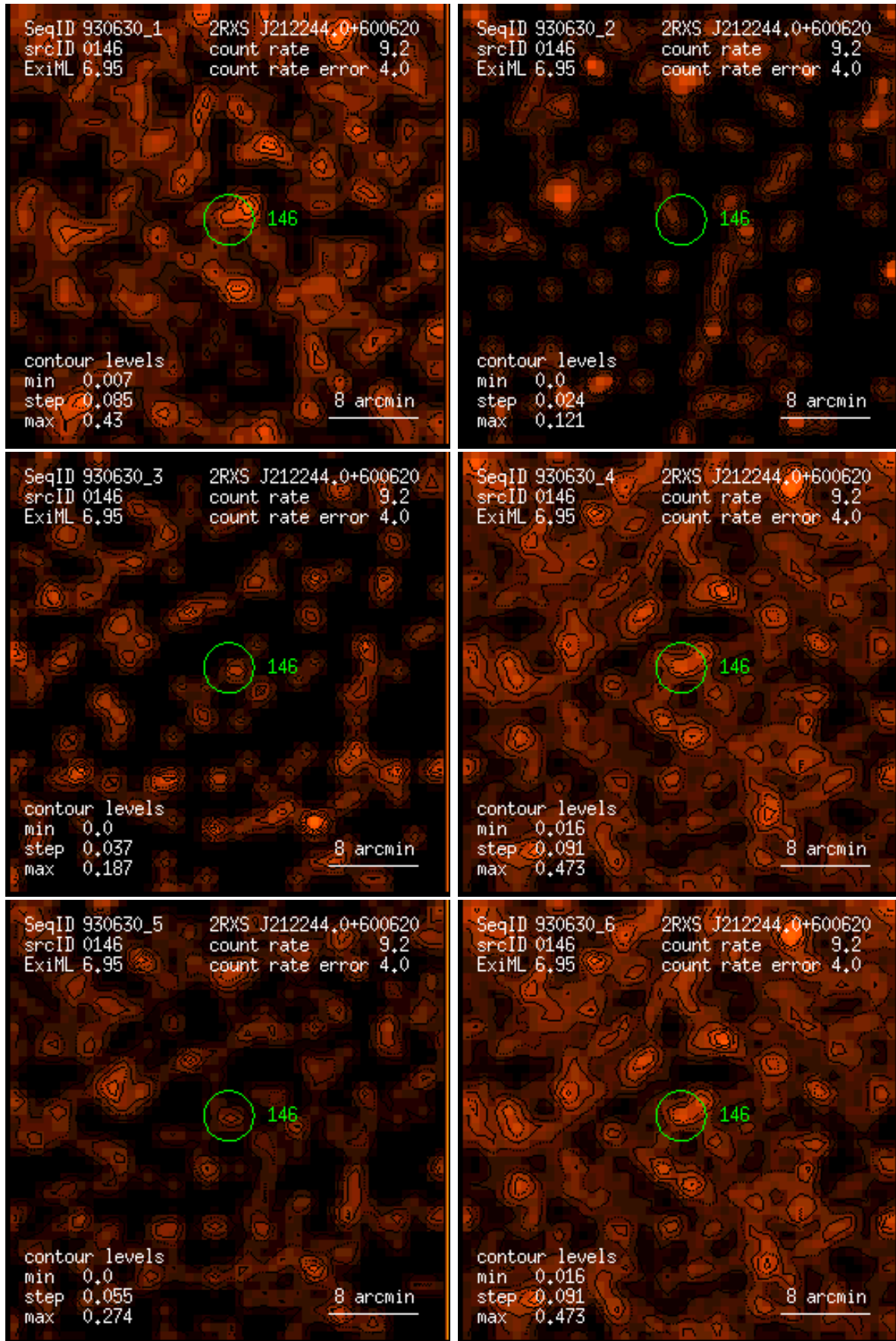
Figure 146: RASS 930630: detection 0146: band rate images, Gaussian filter: (1) PSPC channels 11 – 41, (2) 52 – 90, (3) 91 – 201, (4) 11 – 235, (5) 52 – 201, (6) 11 – 201. Broad band rates in counts/ks. Band rate contour levels in counts/ks/arcmin 2 .
