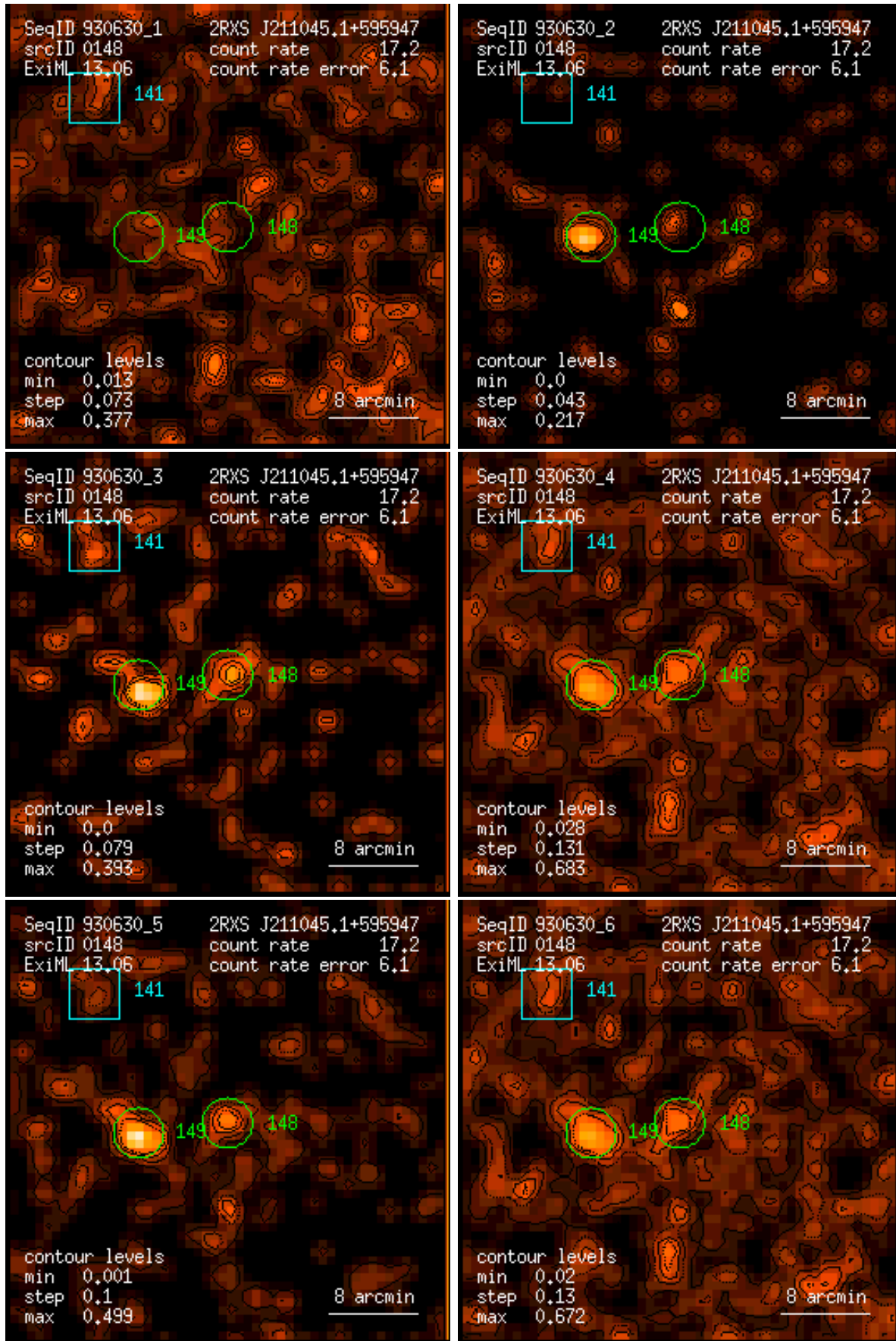
Figure 148: RASS 930630: detection 0148: band rate images, Gaussian filter: (1) PSPC channels 11 – 41, (2) 52 – 90, (3) 91 – 201, (4) 11 – 235, (5) 52 – 201, (6) 11 – 201. Broad band rates in counts/ks. Band rate contour levels in counts/ks/arcmin 2 .
