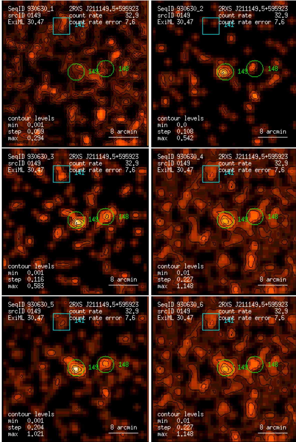
Figure 149: RASS 930630: detection 0149: band rate images, Gaussian filter: (1) PSPC channels 11 – 41, (2) 52 – 90, (3) 91 – 201, (4) 11 – 235, (5) 52 – 201, (6) 11 – 201. Broad band rates in counts/ks. Band rate contour levels in counts/ks/arcmin 2 .
