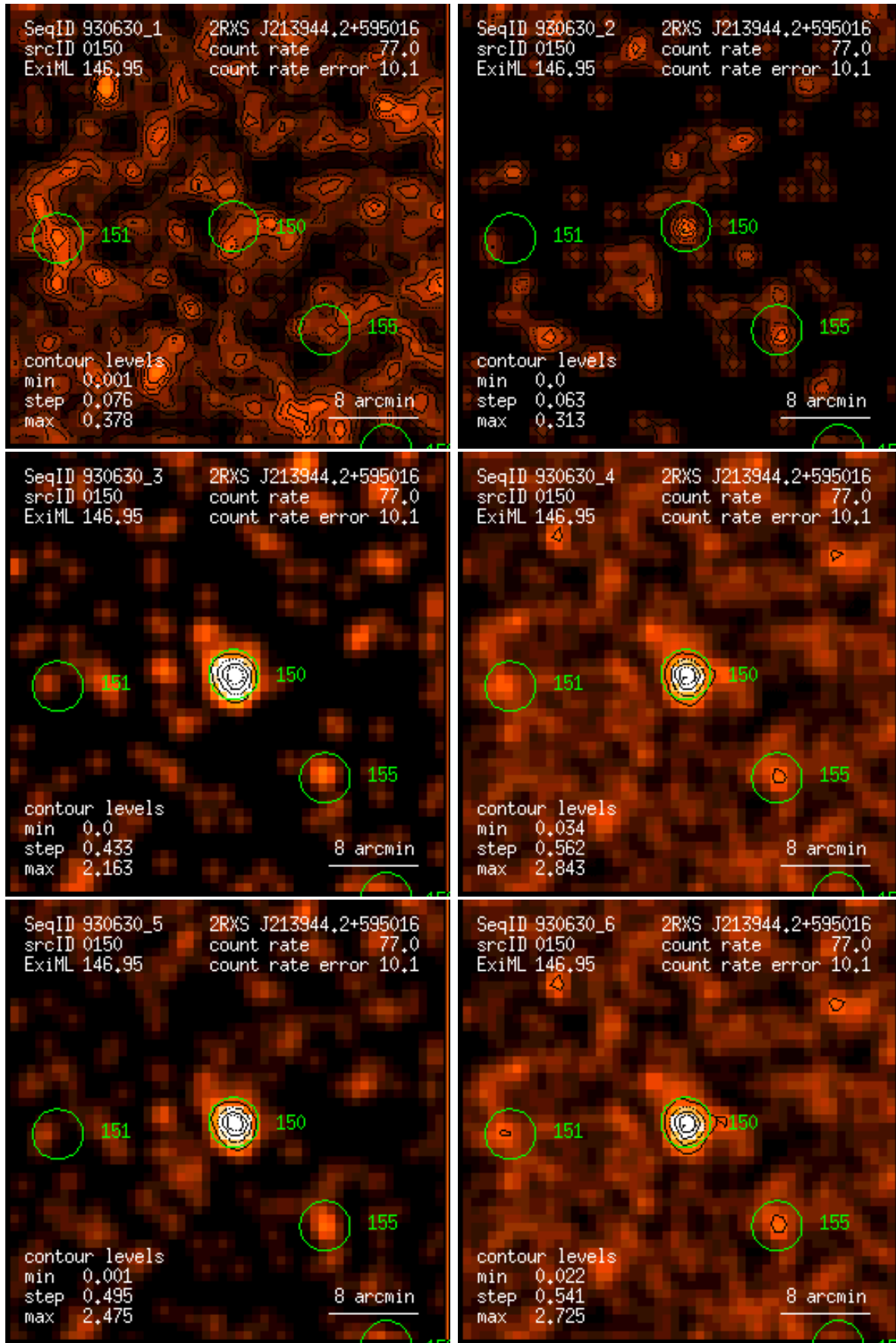
Figure 150: RASS 930630: detection 0150: band rate images, Gaussian filter: (1) PSPC channels 11 – 41, (2) 52 – 90, (3) 91 – 201, (4) 11 – 235, (5) 52 – 201, (6) 11 – 201. Broad band rates in counts/ks. Band rate contour levels in counts/ks/arcmin 2 .
