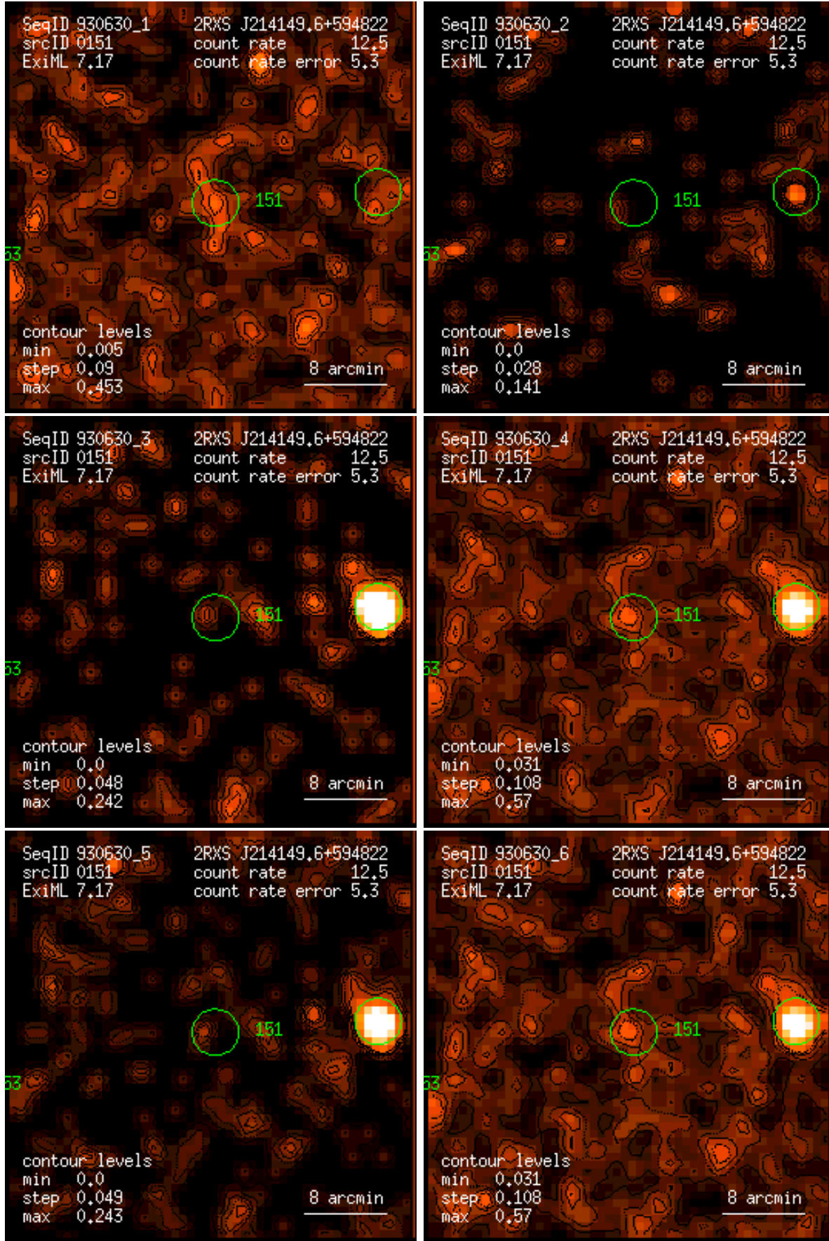
Figure 151: RASS 930630: detection 0151: band rate images, Gaussian filter: (1) PSPC channels 11 – 41, (2) 52 – 90, (3) 91 – 201, (4) 11 – 235, (5) 52 – 201, (6) 11 – 201. Broad band rates in counts/ks. Band rate contour levels in counts/ks/arcmin 2 .
