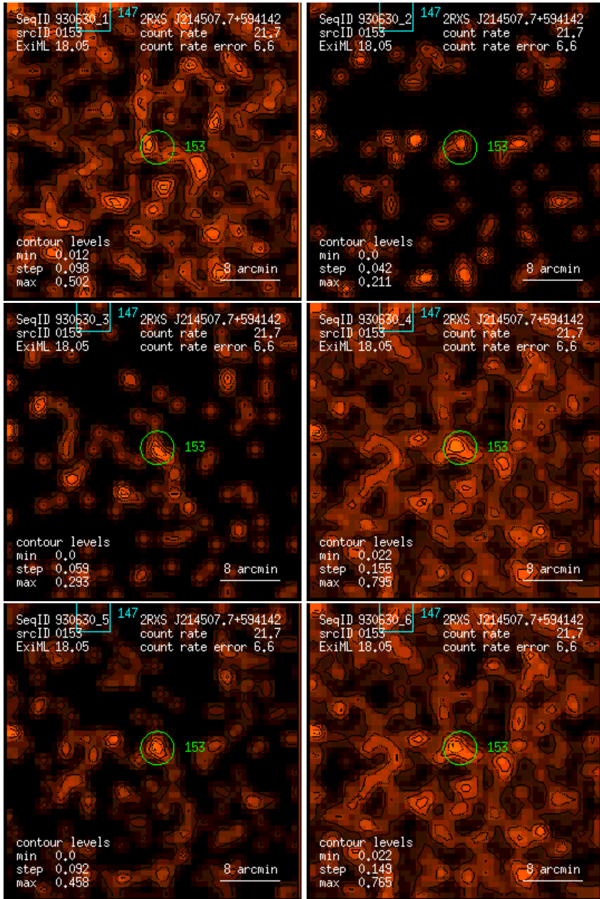
Figure 153: RASS 930630: detection 0153: band rate images, Gaussian filter: (1) PSPC channels 11 – 41, (2) 52 – 90, (3) 91 – 201, (4) 11 – 235, (5) 52 – 201, (6) 11 – 201. Broad band rates in counts/ks. Band rate contour levels in counts/ks/arcmin 2 .
