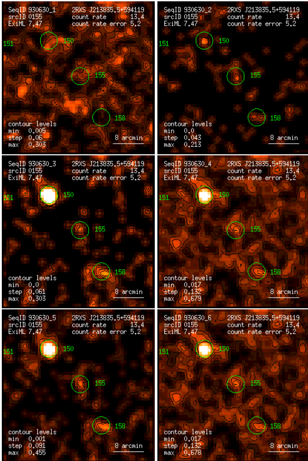
Figure 155: RASS 930630: detection 0155: band rate images, Gaussian filter: (1) PSPC channels 11 – 41, (2) 52 – 90, (3) 91 – 201, (4) 11 – 235, (5) 52 – 201, (6) 11 – 201. Broad band rates in counts/ks. Band rate contour levels in counts/ks/arcmin 2 .
