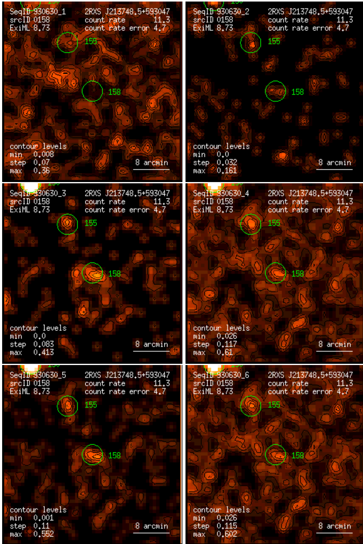
Figure 158: RASS 930630: detection 0158: band rate images, Gaussian filter: (1) PSPC channels 11 – 41, (2) 52 – 90, (3) 91 – 201, (4) 11 – 235, (5) 52 – 201, (6) 11 – 201. Broad band rates in counts/ks. Band rate contour levels in counts/ks/arcmin 2 .
