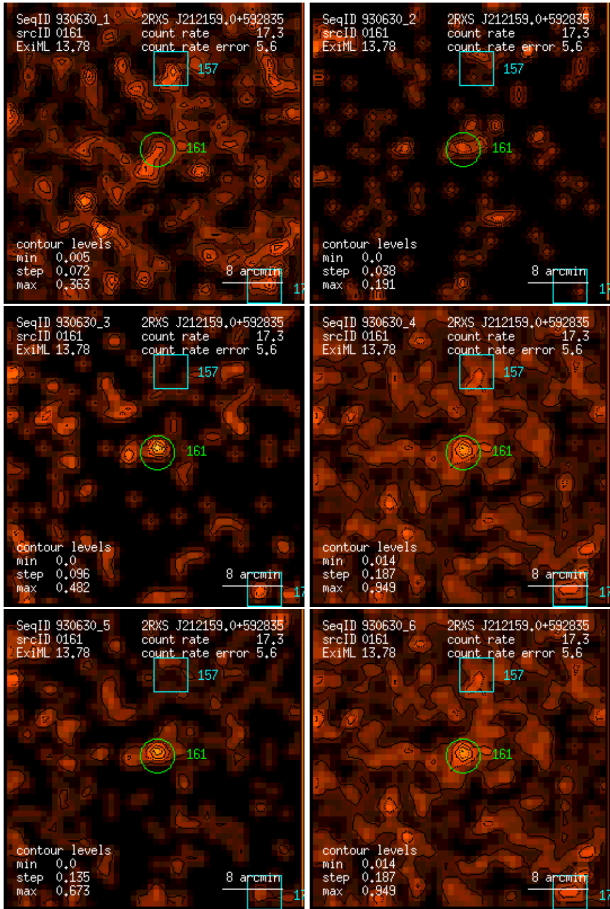
Figure 161: RASS 930630: detection 0161: band rate images, Gaussian filter: (1) PSPC channels 11 – 41, (2) 52 – 90, (3) 91 – 201, (4) 11 – 235, (5) 52 – 201, (6) 11 – 201. Broad band rates in counts/ks. Band rate contour levels in counts/ks/arcmin 2 .
