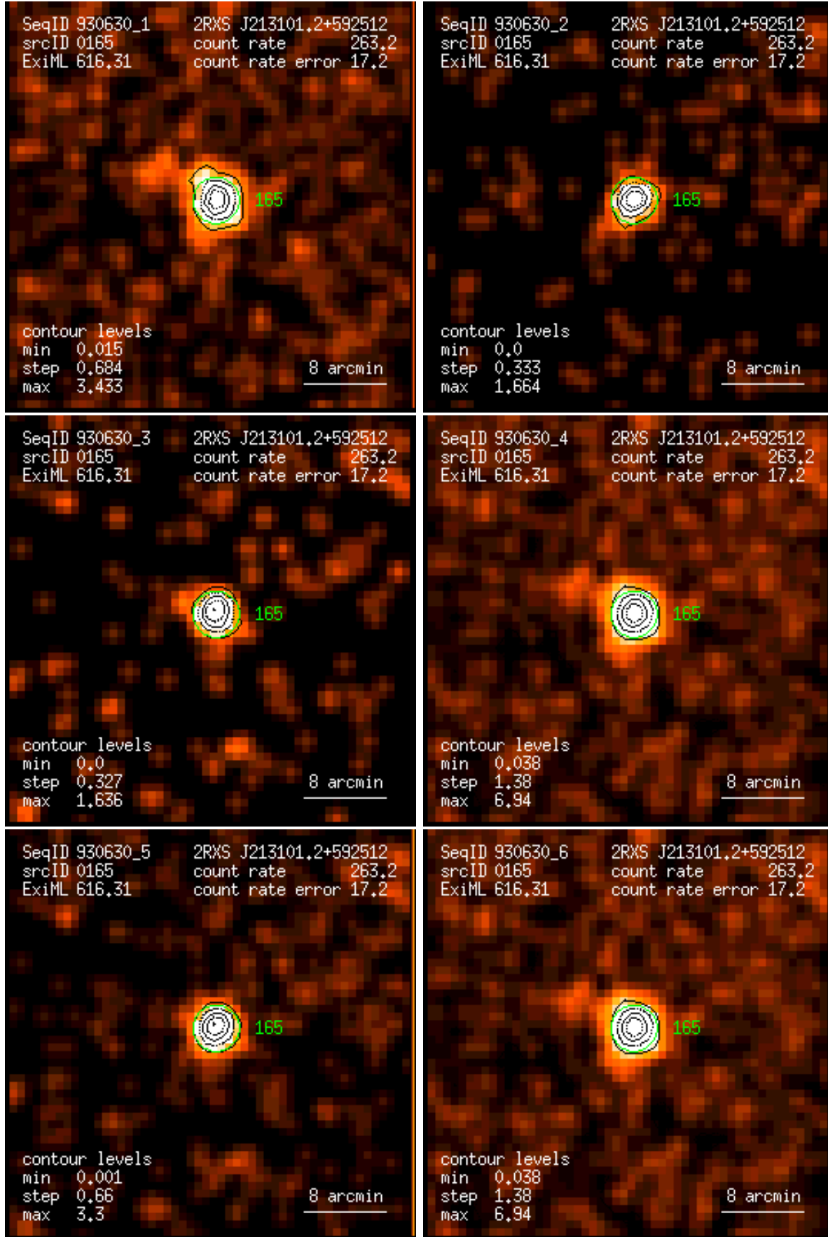
Figure 165: RASS 930630: detection 0165: band rate images, Gaussian filter: (1) PSPC channels 11 – 41, (2) 52 – 90, (3) 91 – 201, (4) 11 – 235, (5) 52 – 201, (6) 11 – 201. Broad band rates in counts/ks. Band rate contour levels in counts/ks/arcmin 2 .
