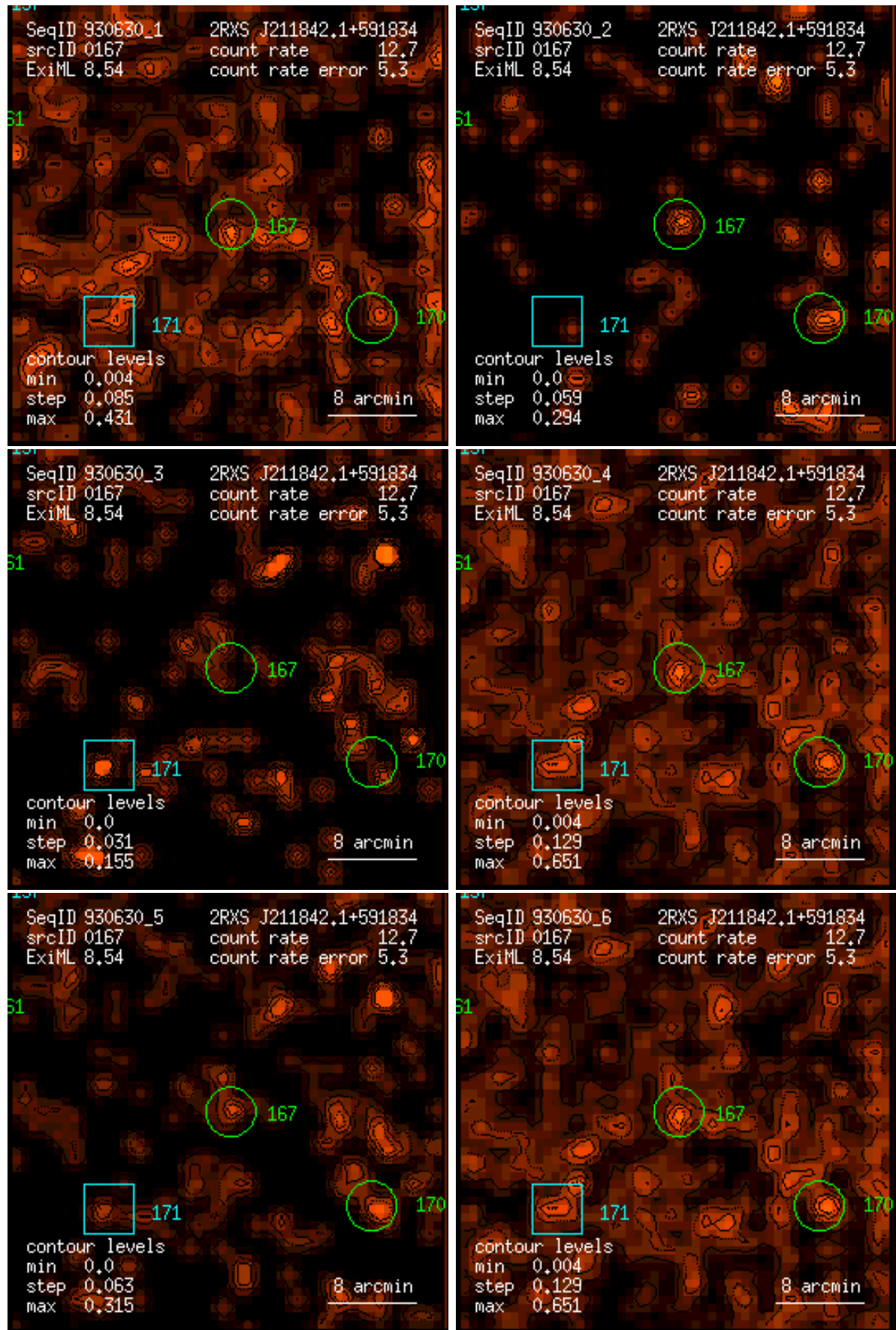
Figure 167: RASS 930630: detection 0167: band rate images, Gaussian filter: (1) PSPC channels 11 – 41, (2) 52 – 90, (3) 91 – 201, (4) 11 – 235, (5) 52 – 201, (6) 11 – 201. Broad band rates in counts/ks. Band rate contour levels in counts/ks/arcmin 2 .
