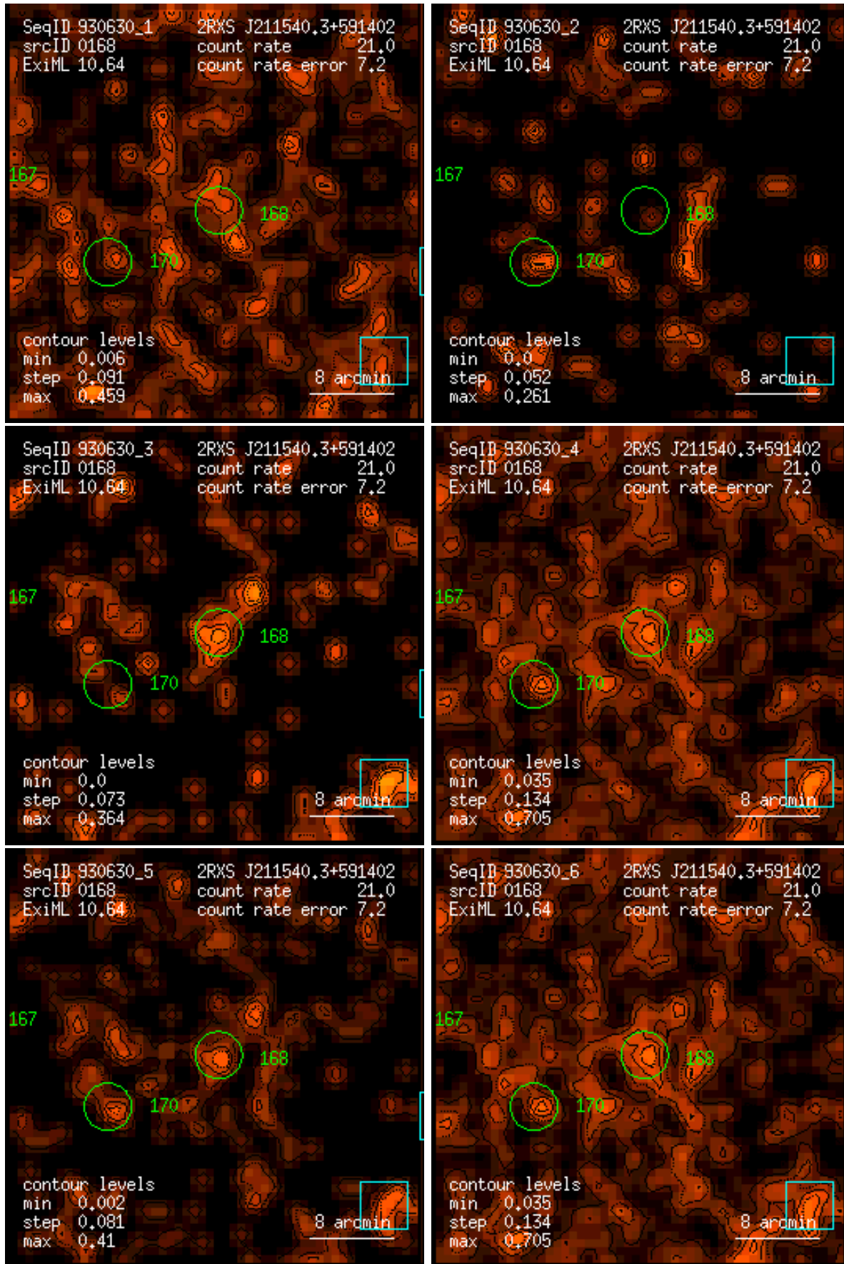
Figure 168: RASS 930630: detection 0168: band rate images, Gaussian filter: (1) PSPC channels 11 – 41, (2) 52 – 90, (3) 91 – 201, (4) 11 – 235, (5) 52 – 201, (6) 11 – 201. Broad band rates in counts/ks. Band rate contour levels in counts/ks/arcmin 2 .
