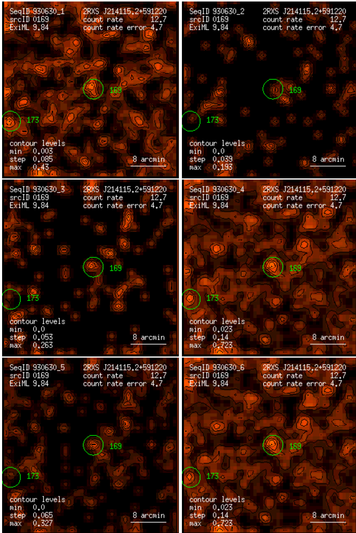
Figure 169: RASS 930630: detection 0169: band rate images, Gaussian filter: (1) PSPC channels 11 – 41, (2) 52 – 90, (3) 91 – 201, (4) 11 – 235, (5) 52 – 201, (6) 11 – 201. Broad band rates in counts/ks. Band rate contour levels in counts/ks/arcmin 2 .
